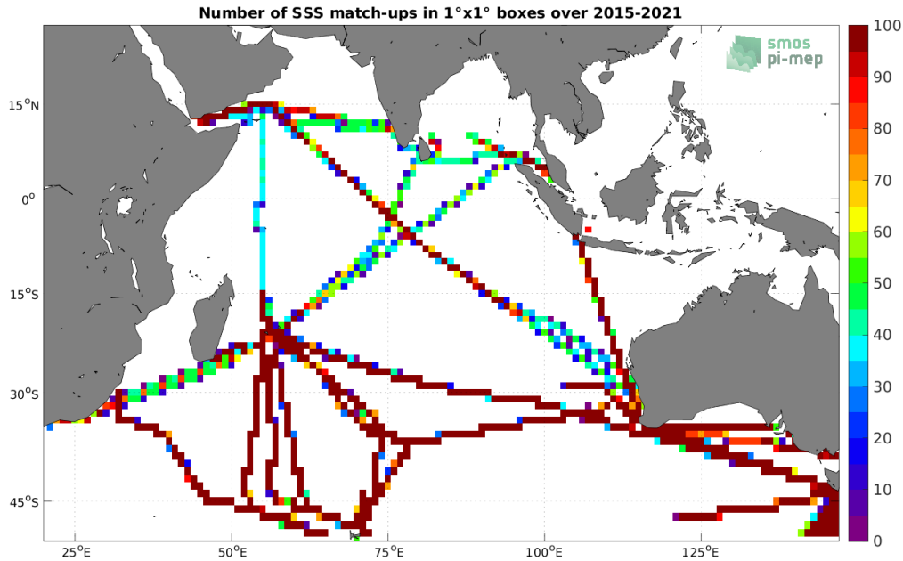
Figure 4: Number of SSS match-ups between TSG (LEGOS-DM) SSS and the SMAP SSS L3 v5 - 8-Day running (RSS) SSS product for the Indian Ocean Pi-MEP region over 1^{\circ} \times 1^{\circ} boxes and for the full satellite product period.
