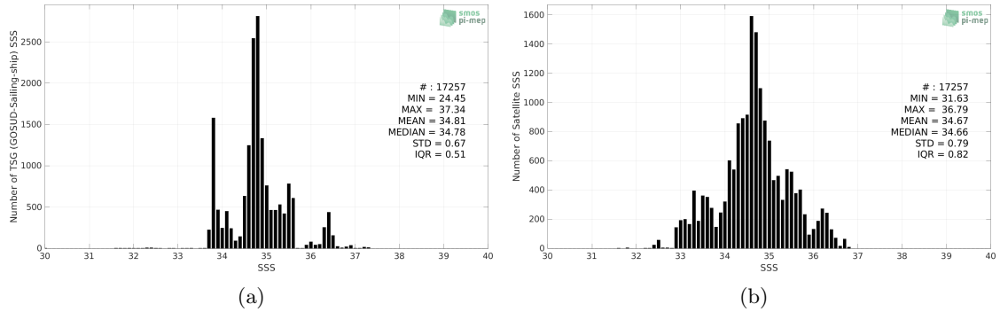
Figure 2: Histograms of SSS from TSG (GOSUD-Sailing-ship) (a) and SMAP SSS L3 v5 - 8-Day running (RSS) (b) considering all match-up pairs per bins of 0.1 over the Indian Ocean Pi-MEP region and for the full satellite product period.
