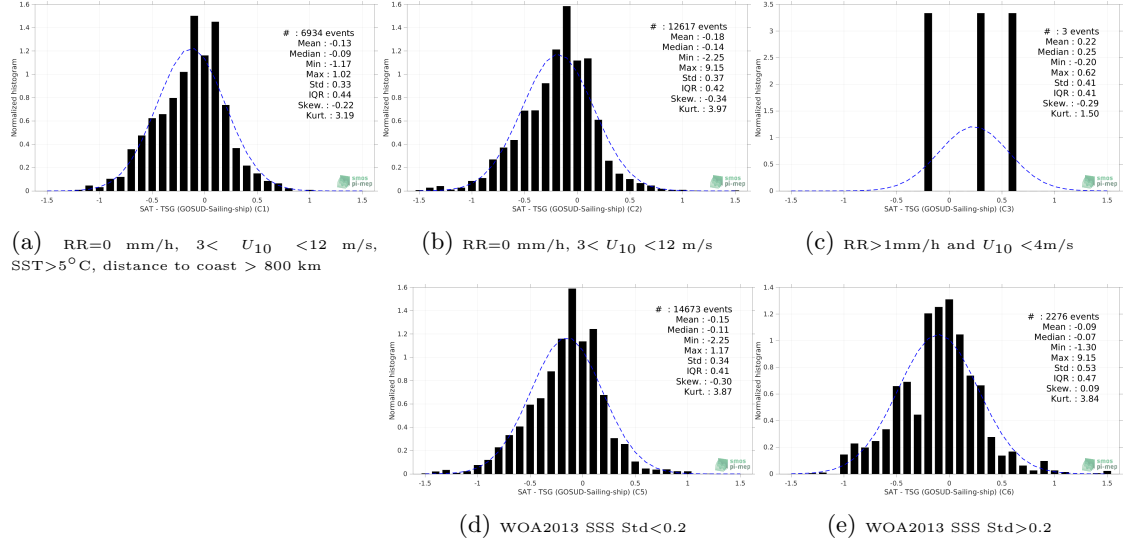
Figure 13: Normalized histogram of \Delta SSS (SMAP SSS L3 v5 - 8-Day running (RSS) - TSG (GOSUD-Sailing-ship)) for 5 different subdatasets corresponding to: RR=0 mm/h, 3 < U_{10} < 12 m/s, SST>5°C, distance to coast > 800 km (a), RR=0 mm/h, 3 < U_{10} < 12 m/s (b), RR>1mm/h and U_{10} < 4 m/s (c), WOA2013 SSS Std<0.2 (d), WOA2013 SSS Std>0.2 (e).
