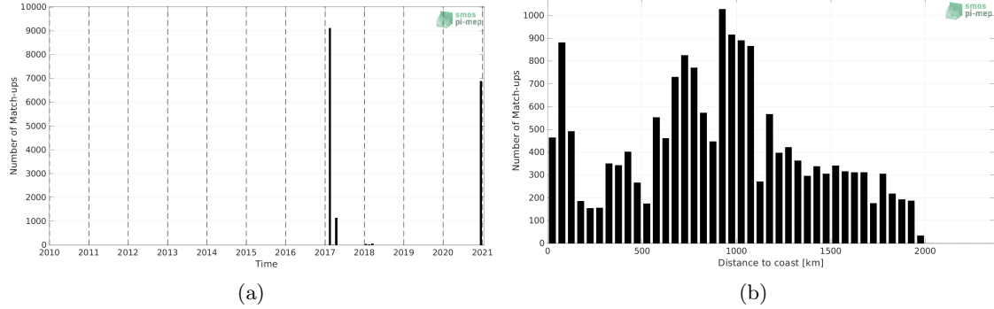
Figure 1: Number of match-ups between TSG (GOSUD-Sailing-ship) and SMAP SSS L3 v5 - 8-Day running (RSS) SSS as a function of time (a) and as function of the distance to coast (b) over the Indian Ocean Pi-MEP region and for the full satellite product period.
