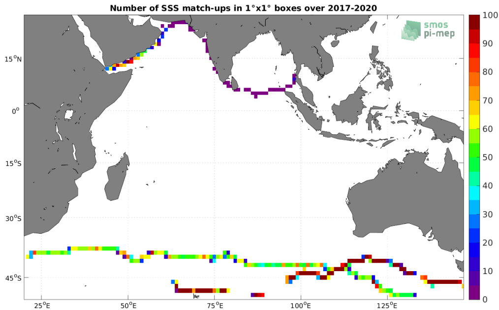
Figure 4: Number of SSS match-ups between TSG (GOSUD-Sailing-ship) SSS and the SMAP SSS L3 v5 - 8-Day running (RSS) SSS product for the Indian Ocean Pi-MEP region over 1^\circ \times 1^\circ boxes and for the full satellite product period.
