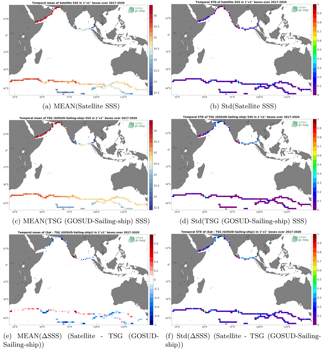
Figure 6: Temporal mean (left) and Std (right) of SSS from SMAP SSS L3 v5 - 8-Day running (RSS) (top), TSG (GOSUD-Sailing-ship) (middle), and of \Delta SSS (Satellite - TSG (GOSUD-Sailing-ship)). Only match-up pairs are used to generate these maps.
