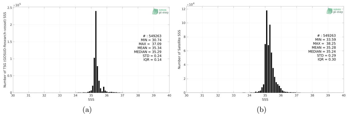
Figure 2: Histograms of SSS from TSG (GOSUD-Research-vessel) (a) and SMAP SSS L3 v5 - 8-Day running (RSS) (b) considering all match-up pairs per bins of 0.1 over the Indian Ocean Pi-MEP region and for the full satellite product period.
