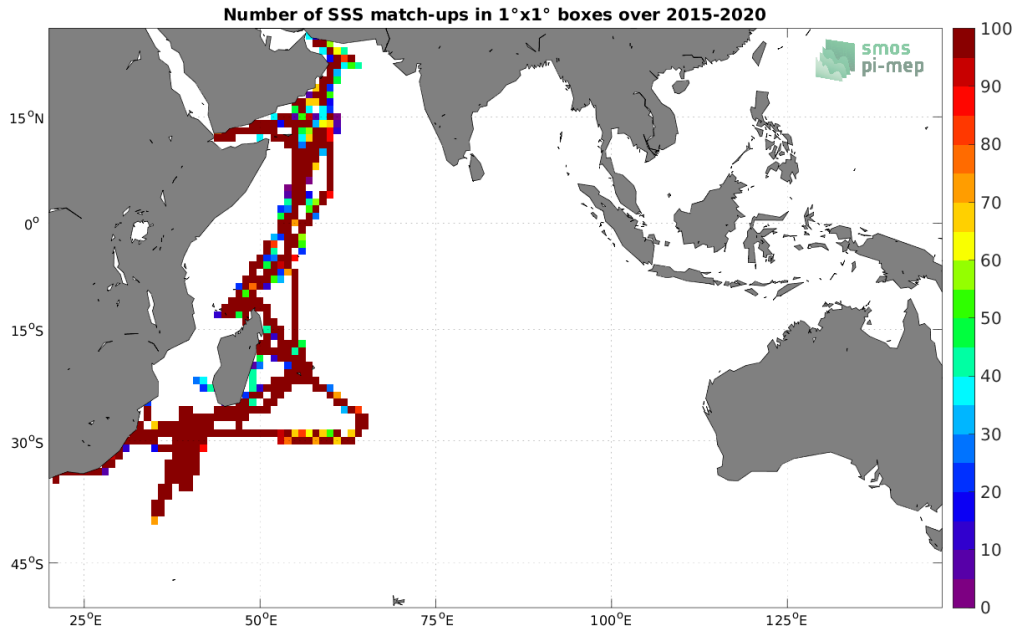
Figure 4: Number of SSS match-ups between TSG (GOSUD-Research-vessel) SSS and the SMAP SSS L3 v5 - 8-Day running (RSS) SSS product for the Indian Ocean Pi-MEP region over 1^\circ \times 1^\circ boxes and for the full satellite product period.
