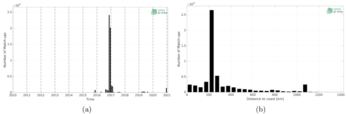
Figure 1: Number of match-ups between TSG (GOSUD-Research-vessel) and SMAP SSS L3 v5 - 8-Day running (RSS) SSS as a function of time (a) and as function of the distance to coast (b) over the Indian Ocean Pi-MEP region and for the full satellite product period.
