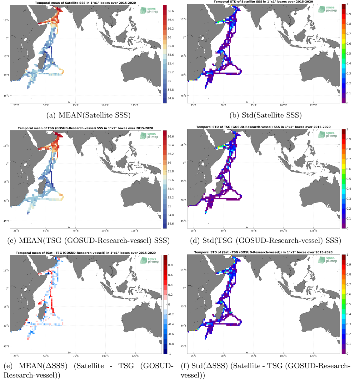
Figure 6: Temporal mean (left) and Std (right) of SSS from SMAP SSS L3 v5 - 8-Day running (RSS) (top), TSG (GOSUD-Research-vessel) (middle), and of \Delta SSS (Satellite - TSG (GOSUD-Research-vessel)). Only match-up pairs are used to generate these maps.
