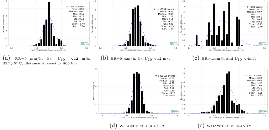
Figure 13: Normalized histogram of \Delta\text{SSS} (SMAP SSS L3 v5 - 8-Day running (RSS) - TSG (GOSUD-Research-vessel)) for 5 different subdatasets corresponding to: RR=0 mm/h, 3 < U_{10} < 12 m/s, SST>5°C, distance to coast > 800 km (a), RR=0 mm/h, 3 < U_{10} < 12 m/s (b), RR>1mm/h and U_{10} < 4 m/s (c), WOA2013 SSS Std<0.2 (d), WOA2013 SSS Std>0.2 (e).
