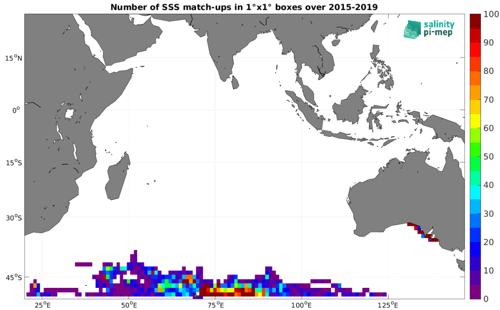
Figure 4: Number of SSS match-ups between Marine mammals SSS and the SMAP SSS L3 v5 - 8-Day running (RSS) SSS product for the Indian Ocean Pi-MEP region over 1^\circ \times 1^\circ boxes and for the full satellite product period.
