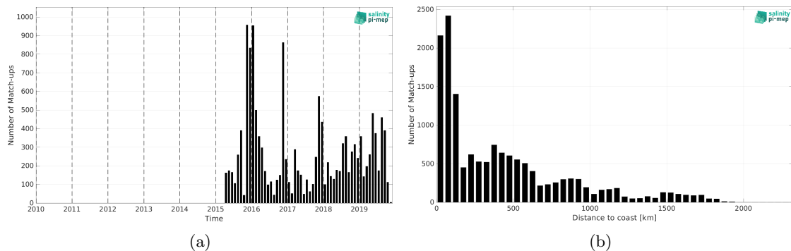
Figure 1: Number of match-ups between Marine mammals and SMAP SSS L3 v5 - 8-Day running (RSS) SSS as a function of time (a) and as function of the distance to coast (b) over the Indian Ocean Pi-MEP region and for the full satellite product period.
