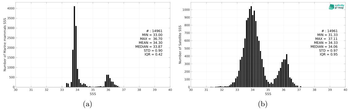
Figure 2: Histograms of SSS from Marine mammals (a) and SMAP SSS L3 v5 - 8-Day running (RSS) (b) considering all match-up pairs per bins of 0.1 over the Indian Ocean Pi-MEP region and for the full satellite product period.
