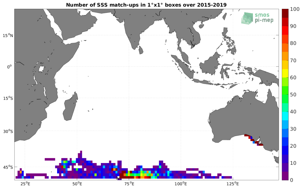
Figure 4: Number of SSS match-ups between Marine mammals SSS and the SMAP SSS L3 v5 - 8-Day running (RSS) SSS product for the Indian Ocean Pi-MEP region over 1^\circ \times 1^\circ boxes and for the full satellite product period.
