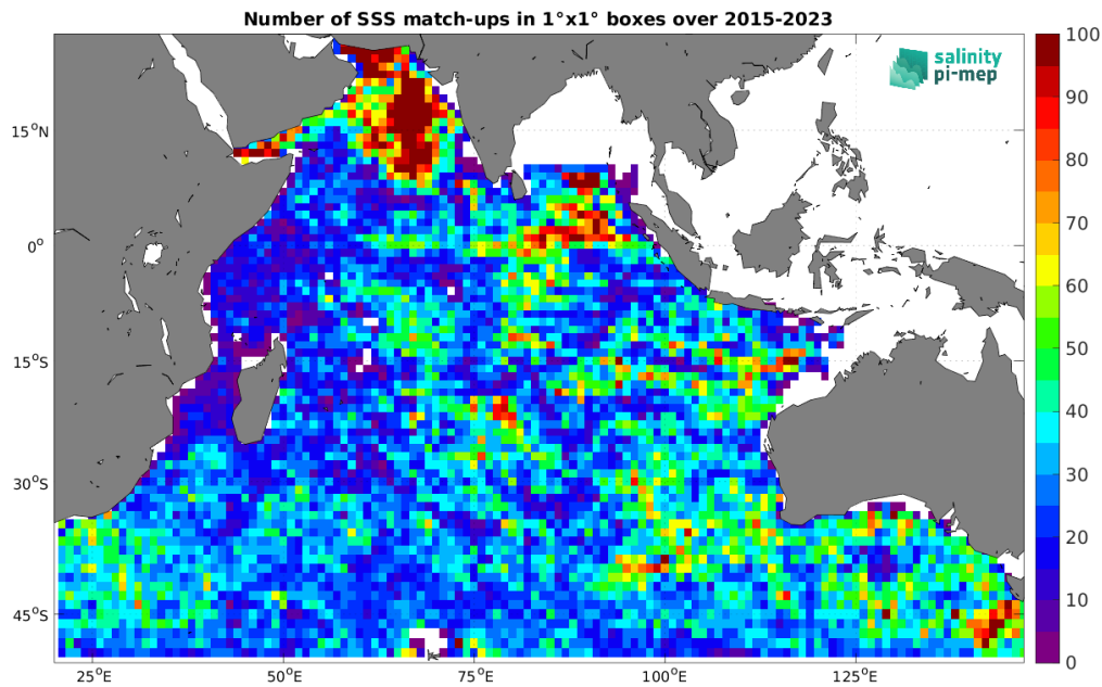
Figure 4: Number of SSS match-ups between Argo SSS and the SMAP SSS L3 v5 - 8-Day running (RSS) SSS product for the Indian Ocean Pi-MEP region over 1^\circ \times 1^\circ boxes and for the full satellite product period.
