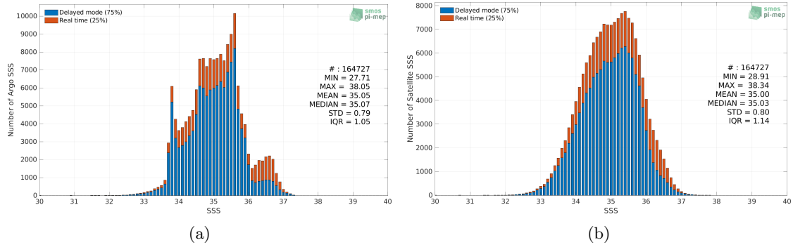
Figure 2: Histograms of SSS from Argo (a) and SMAP SSS L3 v5 - 8-Day running (RSS) (b) considering all match-up pairs per bins of 0.1 over the Indian Ocean Pi-MEP region and for the full satellite product period.
