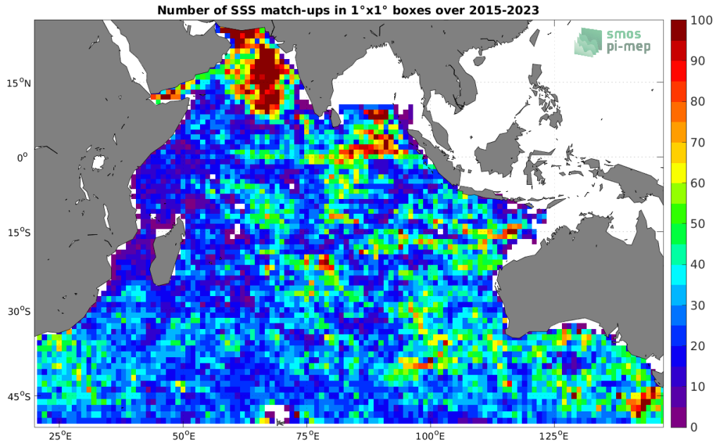
Figure 4: Number of SSS match-ups between Argo SSS and the SMAP SSS L3 v5 - 8-Day running (RSS) SSS product for the Indian Ocean Pi-MEP region over 1^\circ \times 1^\circ boxes and for the full satellite product period.
