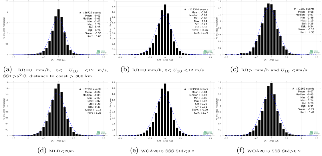
Figure 13: Normalized histogram of \Delta\text{SSS} (SMAP SSS L3 v5 - 8-Day running (RSS) - Argo) for 6 different subdatasets corresponding to: RR=0 mm/h, 3 < U_{10} < 12 m/s, SST>5°C, distance to coast > 800 km (a), RR=0 mm/h, 3 < U_{10} < 12 m/s (b), RR>1mm/h and U_{10} < 4 m/s (c), MLD<20m (d), WOA2013 SSS Std<0.2 (e), WOA2013 SSS Std>0.2 (f).
