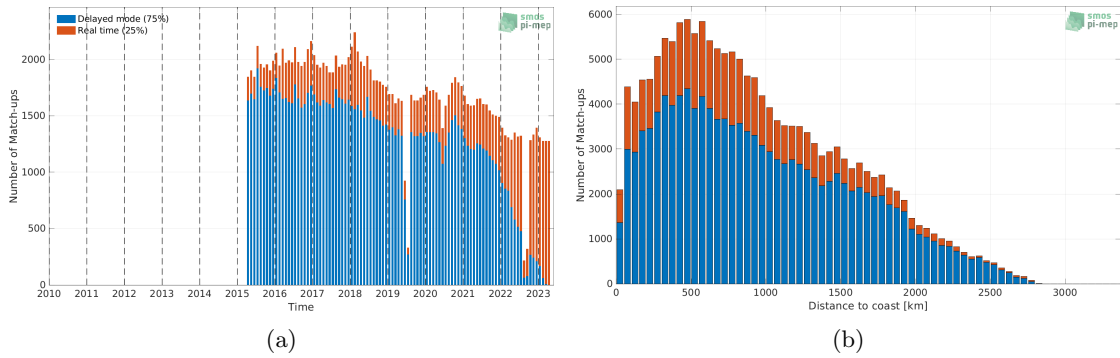
Figure 1: Number of match-ups between Argo and SMAP SSS L3 v5 - 8-Day running (RSS) SSS as a function of time (a) and as function of the distance to coast (b) over the Indian Ocean Pi-MEP region and for the full satellite product period.
