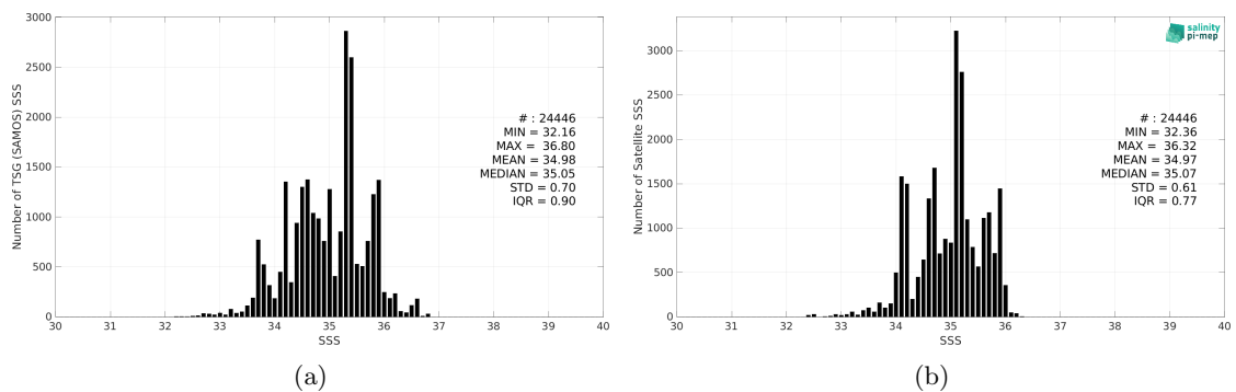
Figure 2: Histograms of SSS from TSG (SAMOS) (a) and SMAP SSS L3 v5 - Monthly (RSS) (b) considering all match-up pairs per bins of 0.1 over the Indian Ocean Pi-MEP region and for the full satellite product period.
