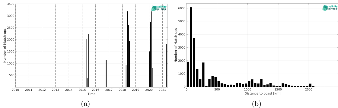
Figure 1: Number of match-ups between TSG (SAMOS) and SMAP SSS L3 v5 - Monthly (RSS) SSS as a function of time (a) and as function of the distance to coast (b) over the Indian Ocean Pi-MEP region and for the full satellite product period.
