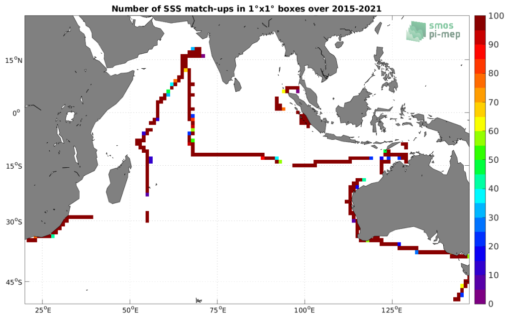
Figure 4: Number of SSS match-ups between TSG (SAMOS) SSS and the SMAP SSS L3 v5 - Monthly (RSS) SSS product for the Indian Ocean Pi-MEP region over 1^\circ \times 1^\circ boxes and for the full satellite product period.
