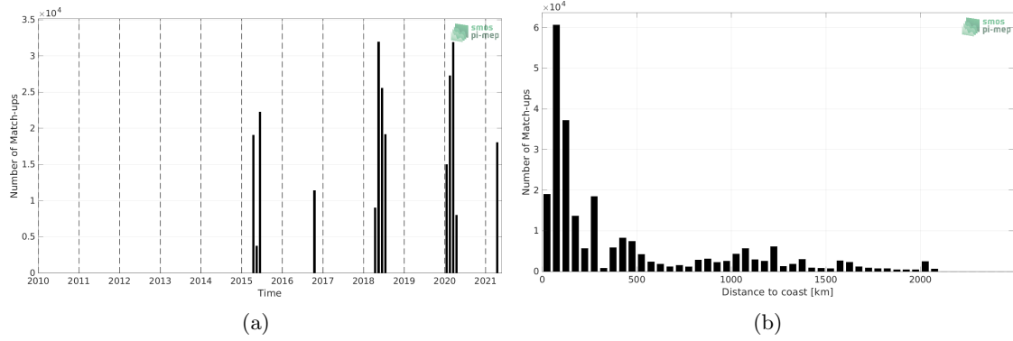
Figure 1: Number of match-ups between TSG (SAMOS) and SMAP SSS L3 v5 - Monthly (RSS) SSS as a function of time (a) and as function of the distance to coast (b) over the Indian Ocean Pi-MEP region and for the full satellite product period.
