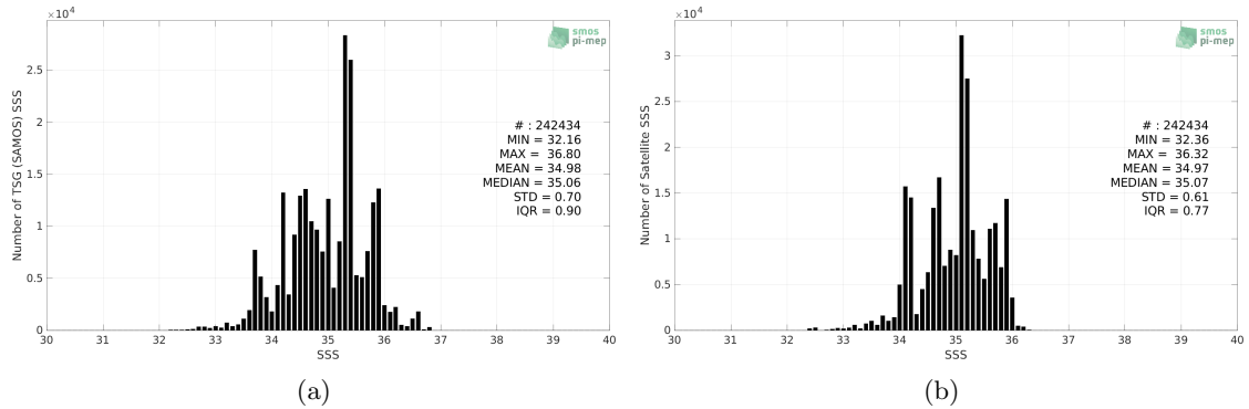
Figure 2: Histograms of SSS from TSG (SAMOS) (a) and SMAP SSS L3 v5 - Monthly (RSS) (b) considering all match-up pairs per bins of 0.1 over the Indian Ocean Pi-MEP region and for the full satellite product period.
