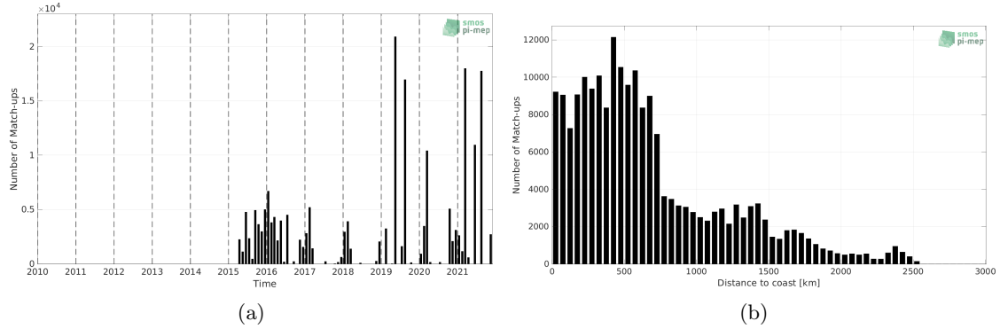
Figure 1: Number of match-ups between TSG (LEGOS-DM) and SMAP SSS L3 v5 - Monthly (RSS) SSS as a function of time (a) and as function of the distance to coast (b) over the Indian Ocean Pi-MEP region and for the full satellite product period.
