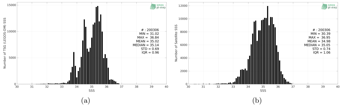
Figure 2: Histograms of SSS from TSG (LEGOS-DM) (a) and SMAP SSS L3 v5 - Monthly (RSS) (b) considering all match-up pairs per bins of 0.1 over the Indian Ocean Pi-MEP region and for the full satellite product period.
