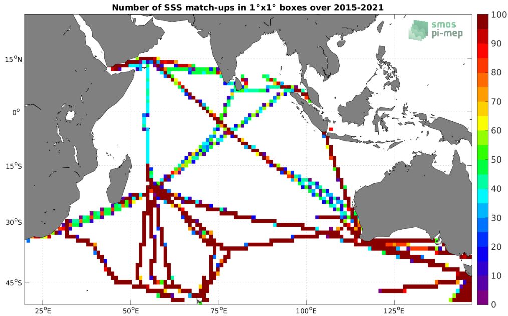
Figure 4: Number of SSS match-ups between TSG (LEGOS-DM) SSS and the SMAP SSS L3 v5 - Monthly (RSS) SSS product for the Indian Ocean Pi-MEP region over 1^\circ \times 1^\circ boxes and for the full satellite product period.
