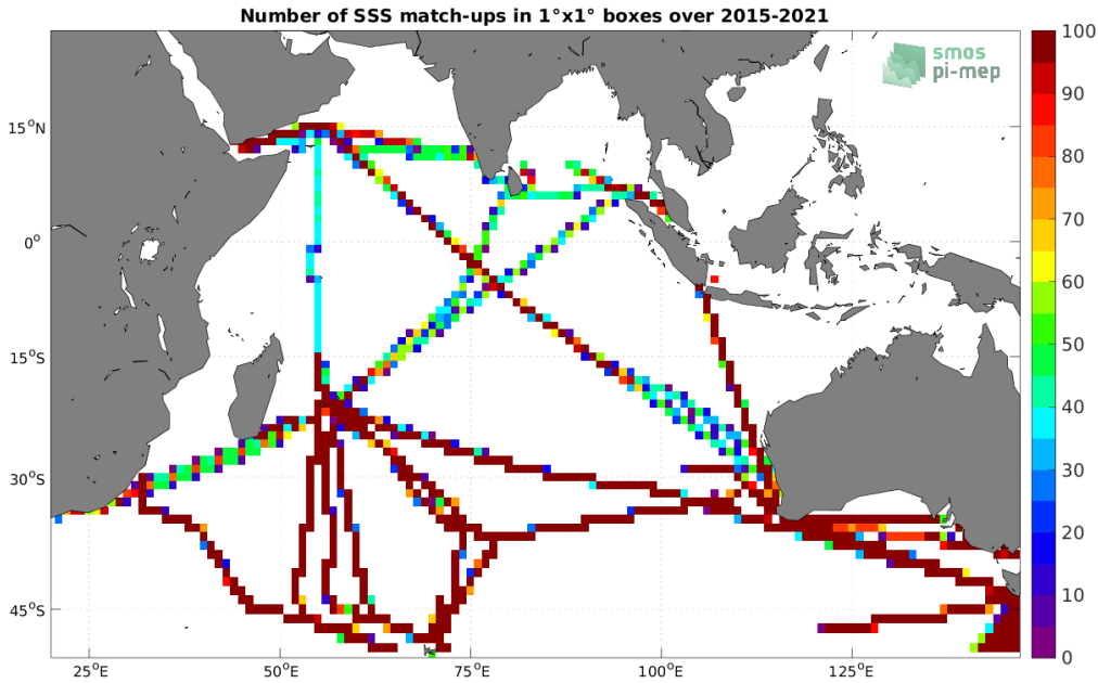
Figure 4: Number of SSS match-ups between TSG (LEGOS-DM) SSS and the SMAP SSS L3 v5 - Monthly (RSS) SSS product for the Indian Ocean Pi-MEP region over 1^\circ \times 1^\circ boxes and for the full satellite product period.
