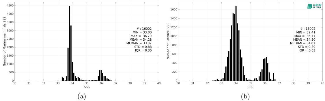
Figure 2: Histograms of SSS from Marine mammals (a) and SMAP SSS L3 v5 - Monthly (RSS) (b) considering all match-up pairs per bins of 0.1 over the Indian Ocean Pi-MEP region and for the full satellite product period.
