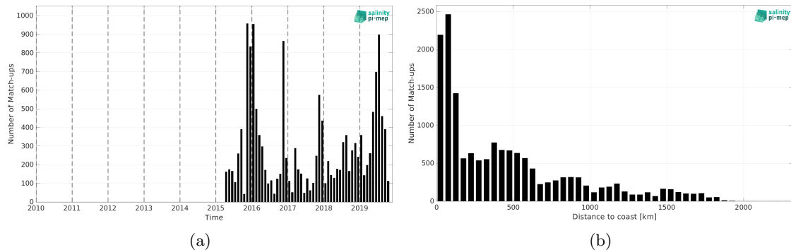
Figure 1: Number of match-ups between Marine mammals and SMAP SSS L3 v5 - Monthly (RSS) SSS as a function of time (a) and as function of the distance to coast (b) over the Indian Ocean Pi-MEP region and for the full satellite product period.
