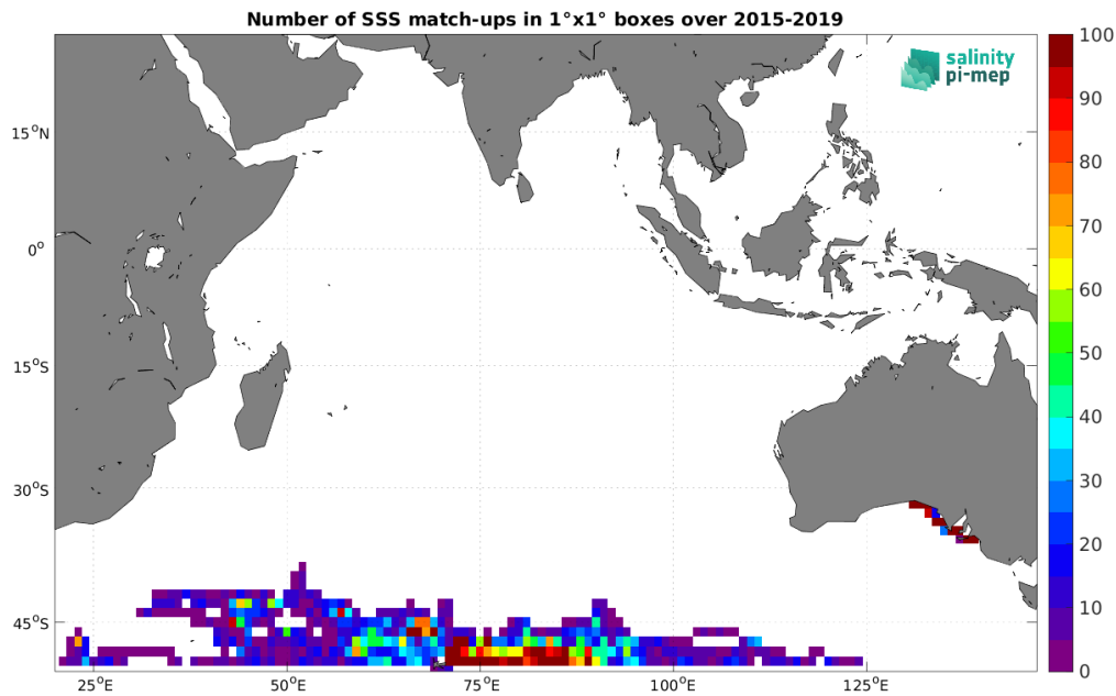
Figure 4: Number of SSS match-ups between Marine mammals SSS and the SMAP SSS L3 v5 - Monthly (RSS) SSS product for the Indian Ocean Pi-MEP region over 1^\circ \times 1^\circ boxes and for the full satellite product period.
