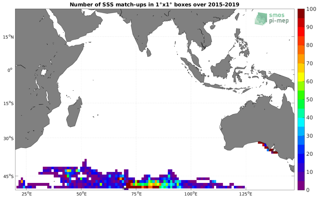
Figure 4: Number of SSS match-ups between Marine mammals SSS and the SMAP SSS L3 v5 - Monthly (RSS) SSS product for the Indian Ocean Pi-MEP region over 1^\circ \times 1^\circ boxes and for the full satellite product period.
