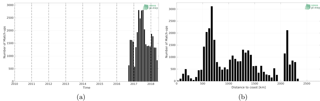
Figure 1: Number of match-ups between Surface drifters and SMAP SSS L3 v5 - Monthly (RSS) SSS as a function of time (a) and as function of the distance to coast (b) over the Indian Ocean Pi-MEP region and for the full satellite product period.
