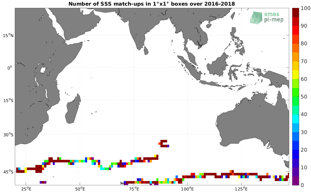
Figure 3: Number of SSS match-ups between Surface drifters SSS and the SMAP SSS L3 v5 - Monthly (RSS) SSS product for the Indian Ocean Pi-MEP region over 1^\circ \times 1^\circ boxes and for the full satellite product period.
