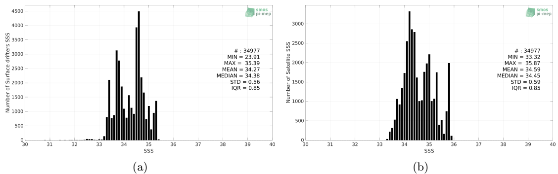
Figure 2: Histograms of SSS from Surface drifters (a) and SMAP SSS L3 v5 - Monthly (RSS) (b) considering all match-up pairs per bins of 0.1 over the Indian Ocean Pi-MEP region and for the full satellite product period.
