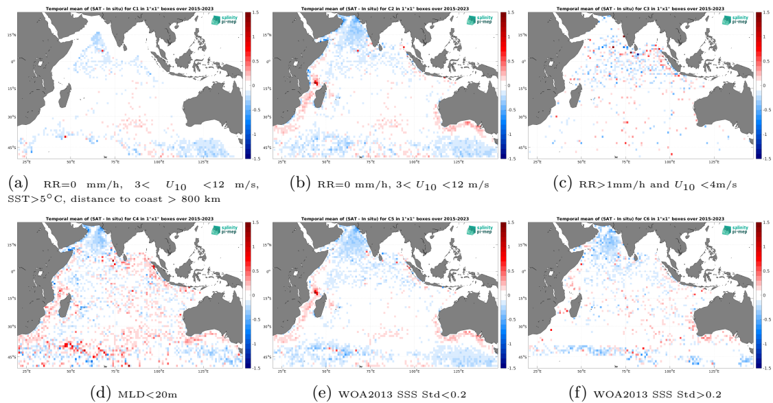
Figure 12: Temporal mean gridded over spatial boxes of size 1^\circ \times 1^\circ of \Delta SSS (SMAP SSS L3 v5 - Monthly (RSS) - Argo) for 6 different subdatasets corresponding to:RR=0 mm/h, 3 < U_{10} < 12 m/s, SST >5^\circ C, distance to coast > 800 km (a), RR=0 mm/h, 3 < U_{10} < 12 m/s (b), RR >1 mm/h and U_{10} < 4 m/s (c),MLD <20 m (d),WOA2013 SSS Std <0.2 (e),WOA2013 SSS Std >0.2 (f).
