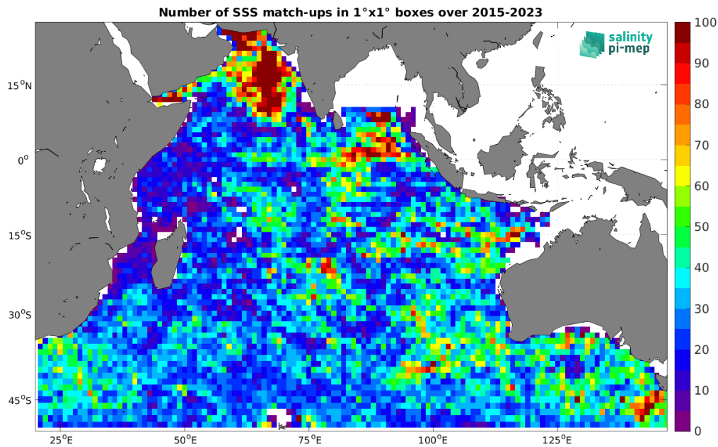
Figure 4: Number of SSS match-ups between Argo SSS and the SMAP SSS L3 v5 - Monthly (RSS) SSS product for the Indian Ocean Pi-MEP region over 1^\circ \times 1^\circ boxes and for the full satellite product period.
