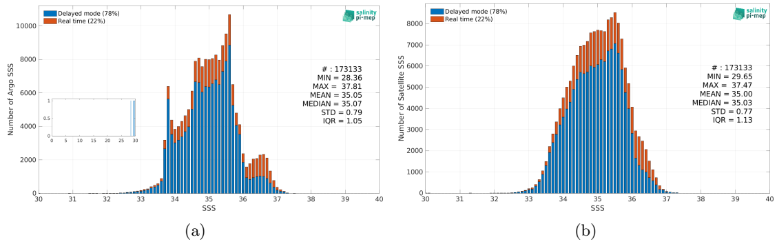
Figure 2: Histograms of SSS from Argo (a) and SMAP SSS L3 v5 - Monthly (RSS) (b) considering all match-up pairs per bins of 0.1 over the Indian Ocean Pi-MEP region and for the full satellite product period.
