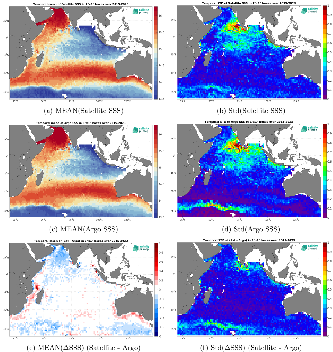
Figure 6: Temporal mean (left) and Std (right) of SSS from SMAP SSS L3 v5 - Monthly (RSS) (top), Argo (middle), and of \Delta SSS (Satellite - Argo). Only match-up pairs are used to generate these maps.
