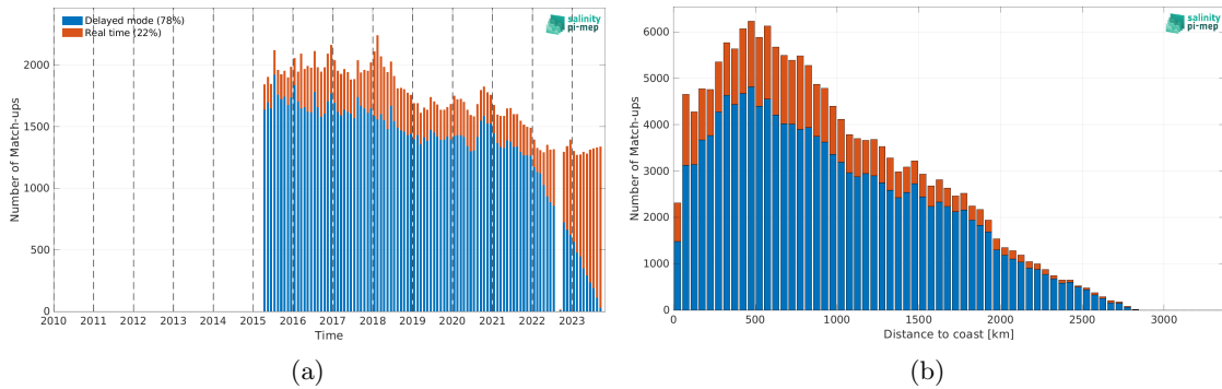
Figure 1: Number of match-ups between Argo and SMAP SSS L3 v5 - Monthly (RSS) SSS as a function of time (a) and as function of the distance to coast (b) over the Indian Ocean Pi-MEP region and for the full satellite product period.
