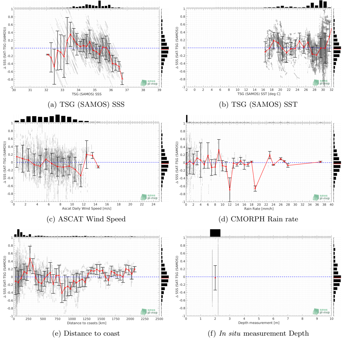
Figure 11: \Delta\text{SSS} (Satellite - TSG (SAMOS)) sorted as function of TSG (SAMOS) SSS values a), TSG (SAMOS) SST b), ASCAT Wind speed c), CMORPH rain rate d), distance to coast (e) and in situ measurement depth (f). In all plots the median and Std of \Delta\text{SSS} for each bin is indicated by the red curves and black vertical thick bars ( \pm 1 Std)
