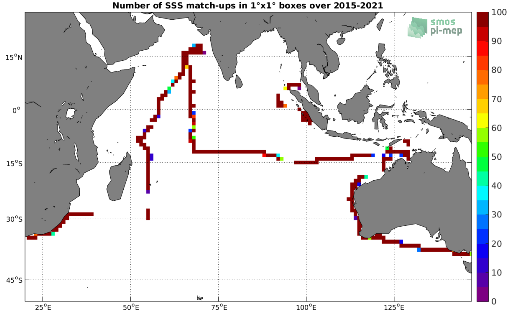
Figure 4: Number of SSS match-ups between TSG (SAMOS) SSS and the SMAP SSS L3 v4 - 8-Day running (RSS) SSS product for the Indian Ocean Pi-MEP region over 1^\circ \times 1^\circ boxes and for the full satellite product period.
