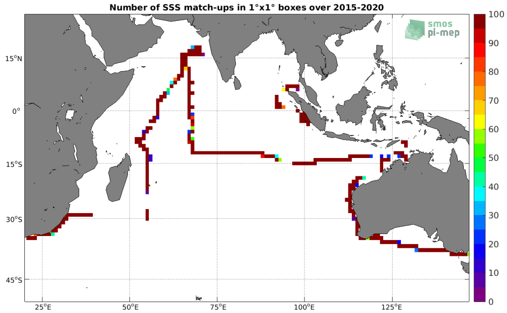
Figure 4: Number of SSS match-ups between TSG (SAMOS) SSS and the SMAP SSS L3 v4 - 8-Day running (RSS) SSS product for the Indian Ocean Pi-MEP region over 1°x1° boxes and for the full satellite product period.
