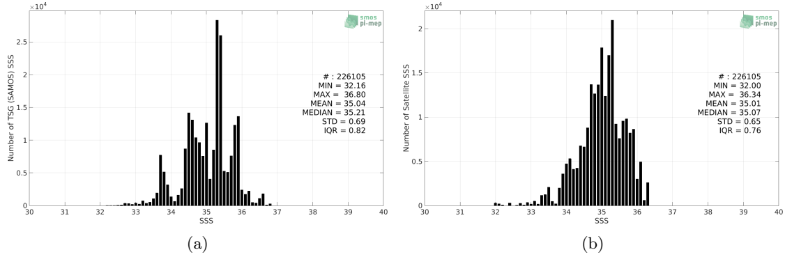
Figure 2: Histograms of SSS from TSG (SAMOS) (a) and SMAP SSS L3 v4 - 8-Day running (RSS) (b) considering all match-up pairs per bins of 0.1 over the Indian Ocean Pi-MEP region and for the full satellite product period.
