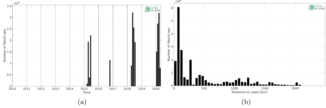
Figure 1: Number of match-ups between TSG (SAMOS) and SMAP SSS L3 v4 - 8-Day running (RSS) SSS as a function of time (a) and as function of the distance to coast (b) over the Indian Ocean Pi-MEP region and for the full satellite product period.
