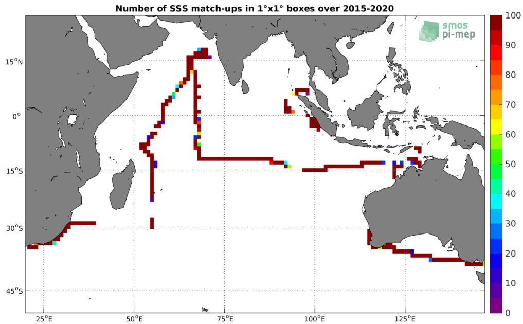
Figure 4: Number of SSS match-ups between TSG-SAMOS SSS and the SMAP-L3-RSS-V4-8DAY-RUNNING SSS product for the Indian Ocean Pi-MEP region over 1^\circ \times 1^\circ boxes and for the full satellite product period.
