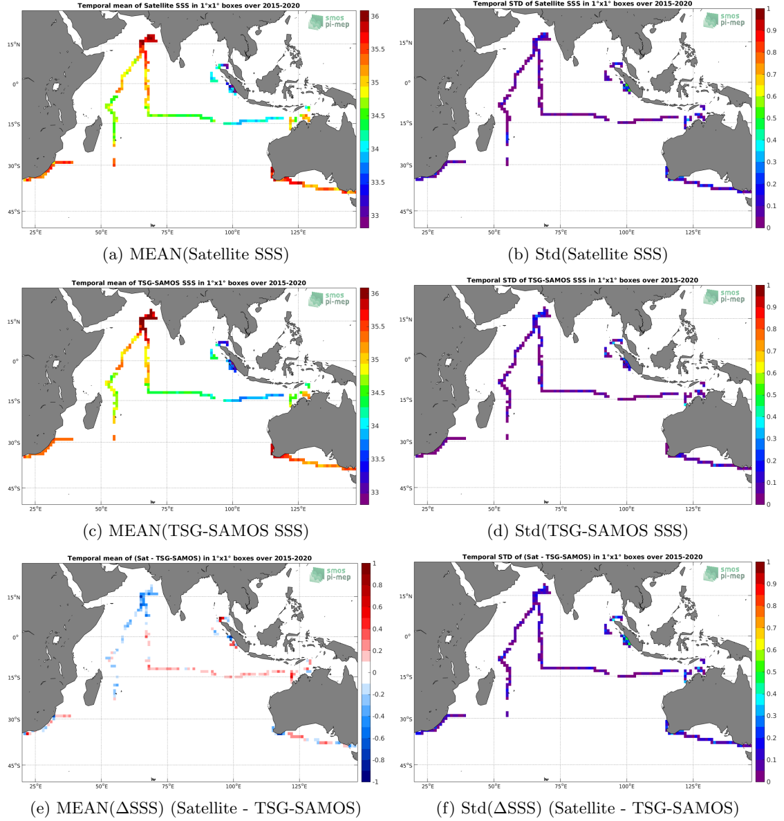
Figure 6: Temporal mean (left) and Std (right) of SSS from SMAP-L3-RSS-V4-8DAY-RUNNING (top), TSG-SAMOS (middle), and of \Delta SSS (Satellite - TSG-SAMOS). Only match-up pairs are used to generate these maps.
