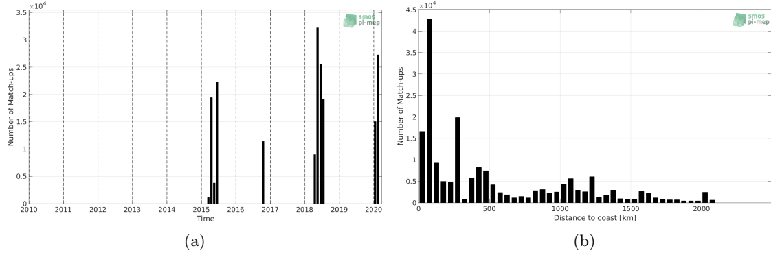
Figure 1: Number of match-ups between TSG-SAMOS and SMAP-L3-RSS-V4-8DAY-RUNNING SSS as a function of time (a) and as function of the distance to coast (b) over the Indian Ocean Pi-MEP region and for the full satellite product period.
