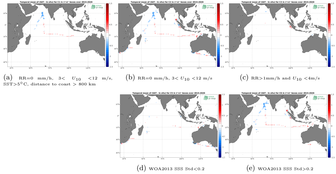
Figure 12: Temporal mean gridded over spatial boxes of size 1^\circ \times 1^\circ of \Delta SSS (SMAP-L3-RSS-V4-8DAY-RUNNING - TSG-SAMOS) for 5 different subdatasets corresponding to: RR=0 mm/h, 3 < U_{10} < 12 m/s, SST > 5^\circ\text{C} , distance to coast > 800 km (a), RR=0 mm/h, 3 < U_{10} < 12 m/s (b), RR > 1 mm/h and U_{10} < 4 m/s (c), WOA2013 SSS Std < 0.2 (d), WOA2013 SSS Std > 0.2 (e).
