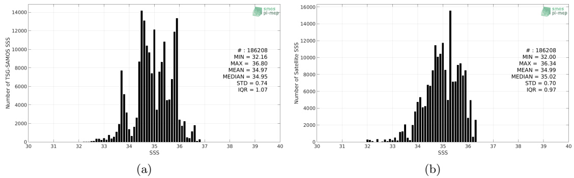
Figure 2: Histograms of SSS from TSG-SAMOS (a) and SMAP-L3-RSS-V4-8DAY-RUNNING (b) considering all match-up pairs per bins of 0.1 over the Indian Ocean Pi-MEP region and for the full satellite product period.
