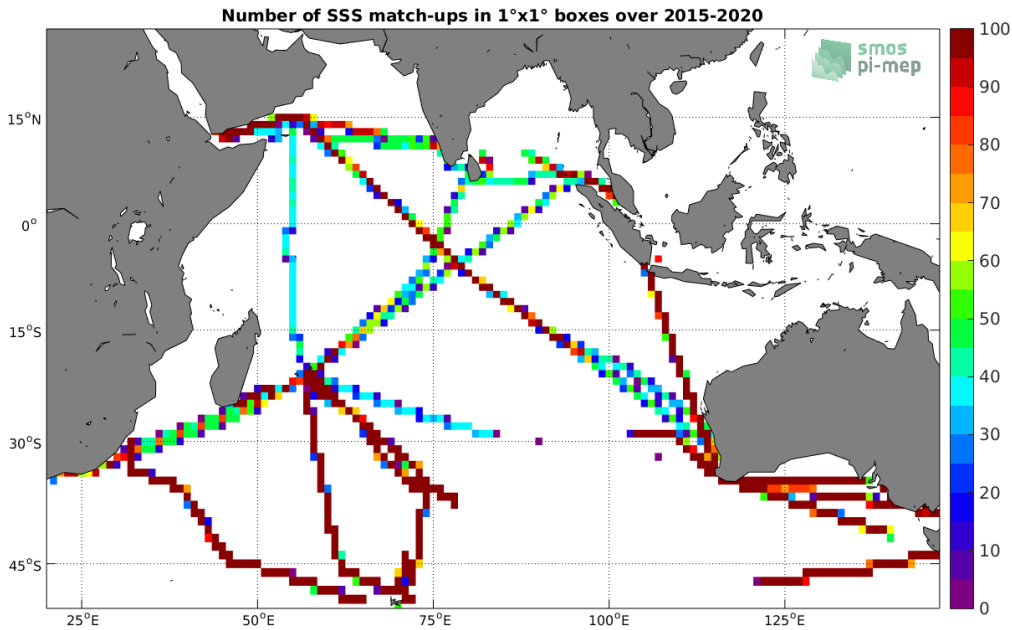
Figure 4: Number of SSS match-ups between TSG (LEGOS-DM) SSS and the SMAP SSS L3 v4 - 8-Day running (RSS) SSS product for the Indian Ocean Pi-MEP region over 1^\circ \times 1^\circ boxes and for the full satellite product period.
