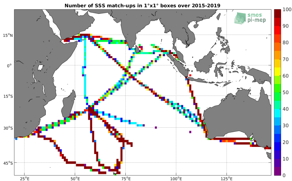
Figure 4: Number of SSS match-ups between TSG-LEGOS-DM SSS and the SMAP-L3-RSS-V4-8DAY-RUNNING SSS product for the Indian Ocean Pi-MEP region over 1^\circ \times 1^\circ boxes and for the full satellite product period.
