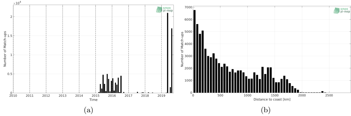
Figure 1: Number of match-ups between TSG-LEGOS-DM and SMAP-L3-RSS-V4-8DAY-RUNNING SSS as a function of time (a) and as function of the distance to coast (b) over the Indian Ocean Pi-MEP region and for the full satellite product period.
