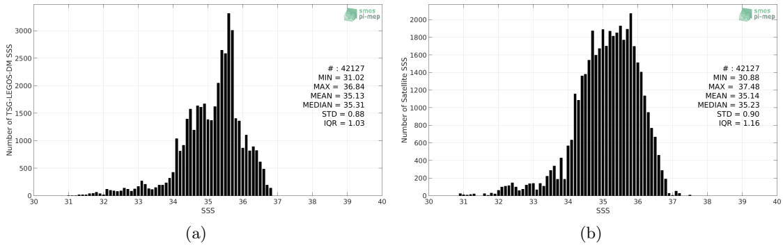
Figure 2: Histograms of SSS from TSG-LEGOS-DM (a) and SMAP-L3-RSS-V4-8DAY-RUNNING (b) considering all match-up pairs per bins of 0.1 over the Indian Ocean Pi-MEP region and for the full satellite product period.
