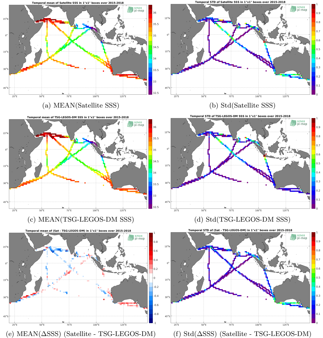
Figure 6: Temporal mean (left) and Std (right) of SSS from SMAP-L3-RSS-V4-8DAY-RUNNING (top), TSG-LEGOS-DM (middle), and of \Delta SSS (Satellite - TSG-LEGOS-DM). Only match-up pairs are used to generate these maps.
