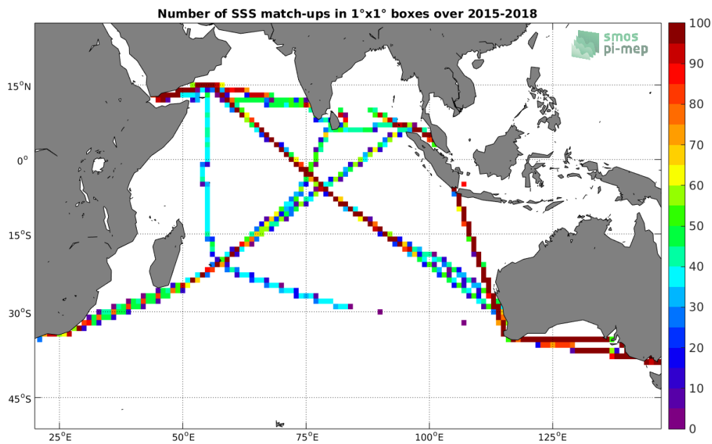
Figure 4: Number of SSS match-ups between TSG-LEGOS-DM SSS and the SMAP-L3-RSS-V4-8DAY-RUNNING SSS product for the Indian Ocean Pi-MEP region over 1^\circ \times 1^\circ boxes and for the full satellite product period.
