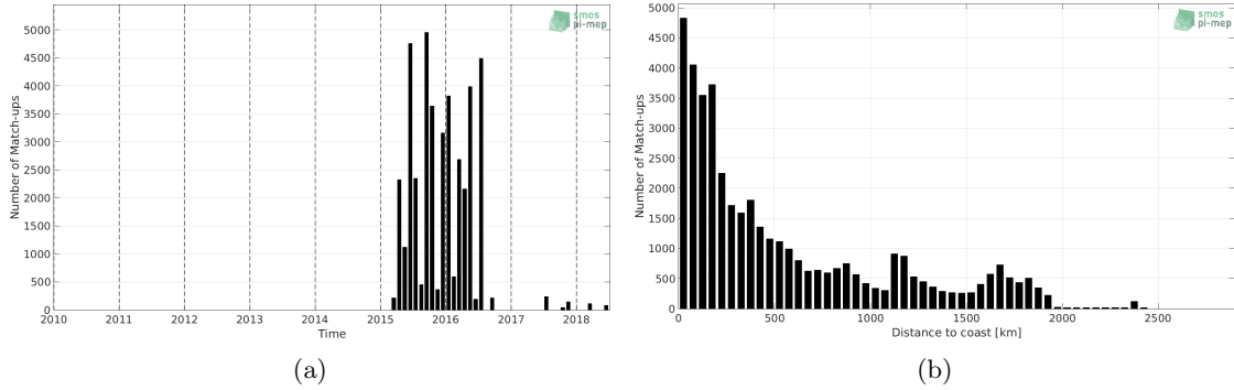
Figure 1: Number of match-ups between TSG-LEGOS-DM and SMAP-L3-RSS-V4-8DAY-RUNNING SSS as a function of time (a) and as function of the distance to coast (b) over the Indian Ocean Pi-MEP region and for the full satellite product period.
