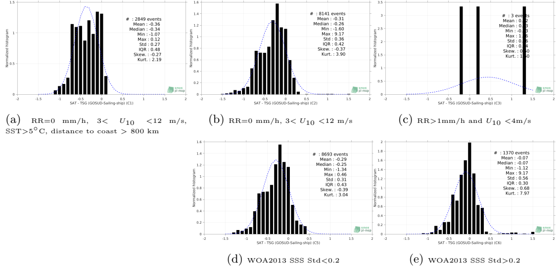
Figure 13: Normalized histogram of \Delta\text{SSS} (SMAP SSS L3 v4 - 8-Day running (RSS) - TSG (GOSUD-Sailing-ship)) for 5 different subdatasets corresponding to: RR=0 mm/h, 3 < U_{10} < 12 m/s, SST > 5^\circ\text{C} , distance to coast > 800 km (a), RR=0 mm/h, 3 < U_{10} < 12 m/s (b), RR > 1\text{mm/h} and U_{10} < 4\text{m/s} (c), WOA2013 SSS Std < 0.2 (d), WOA2013 SSS Std > 0.2 (e).
