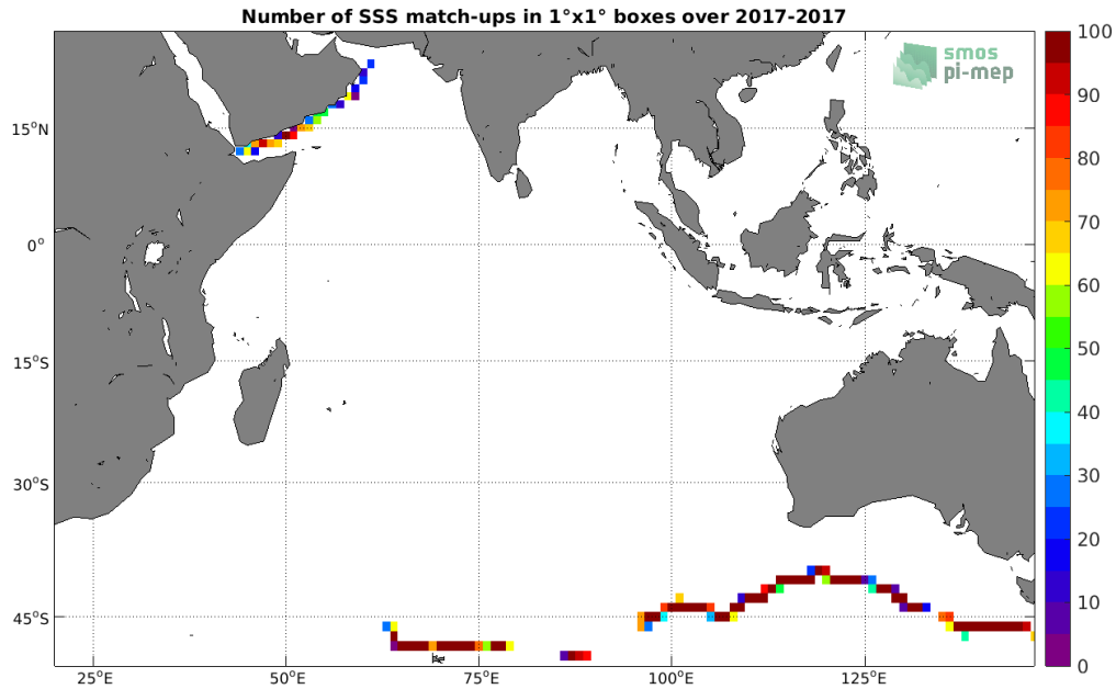
Figure 4: Number of SSS match-ups between TSG (GOSUD-Sailing-ship) SSS and the SMAP SSS L3 v4 - 8-Day running (RSS) SSS product for the Indian Ocean Pi-MEP region over 1°x1° boxes and for the full satellite product period.
