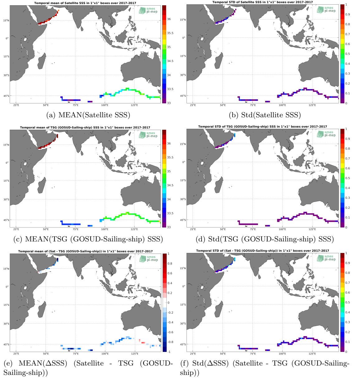
Figure 6: Temporal mean (left) and Std (right) of SSS from SMAP SSS L3 v4 - 8-Day running (RSS) (top), TSG (GOSUD-Sailing-ship) (middle), and of \Delta SSS (Satellite - TSG (GOSUD-Sailing-ship)). Only match-up pairs are used to generate these maps.
