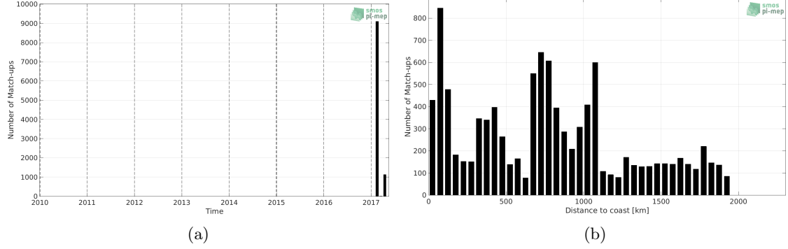
Figure 1: Number of match-ups between TSG (GOSUD-Sailing-ship) and SMAP SSS L3 v4 - 8-Day running (RSS) SSS as a function of time (a) and as function of the distance to coast (b) over the Indian Ocean Pi-MEP region and for the full satellite product period.
