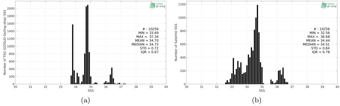
Figure 2: Histograms of SSS from TSG (GOSUD-Sailing-ship) (a) and SMAP SSS L3 v4 - 8-Day running (RSS) (b) considering all match-up pairs per bins of 0.1 over the Indian Ocean Pi-MEP region and for the full satellite product period.
