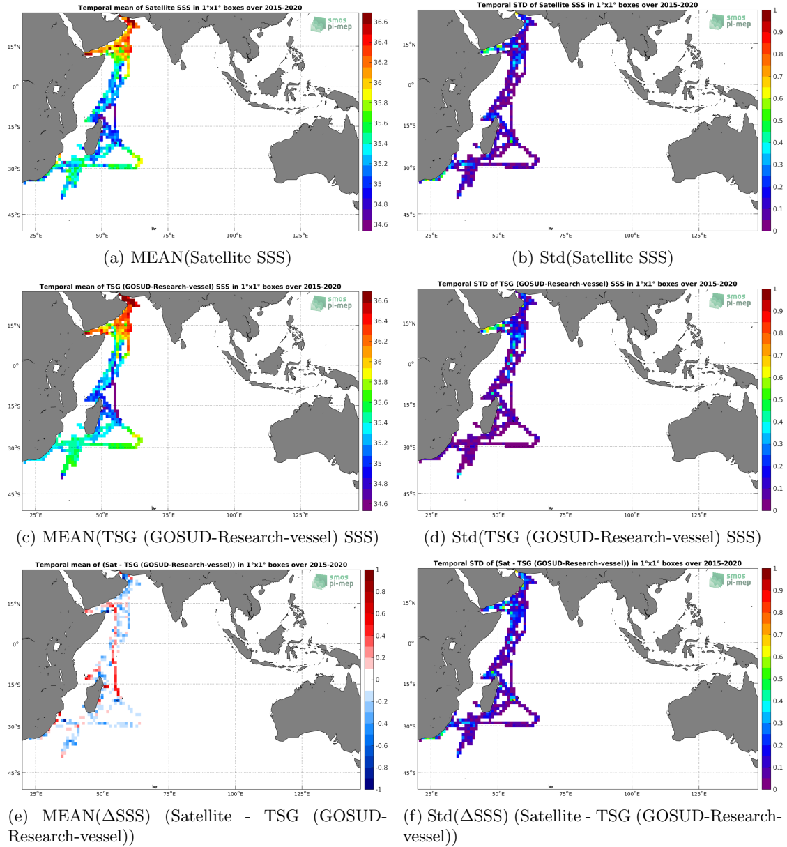
Figure 6: Temporal mean (left) and Std (right) of SSS from SMAP SSS L3 v4 - 8-Day running (RSS) (top), TSG (GOSUD-Research-vessel) (middle), and of \Delta SSS (Satellite - TSG (GOSUD-Research-vessel)). Only match-up pairs are used to generate these maps.
