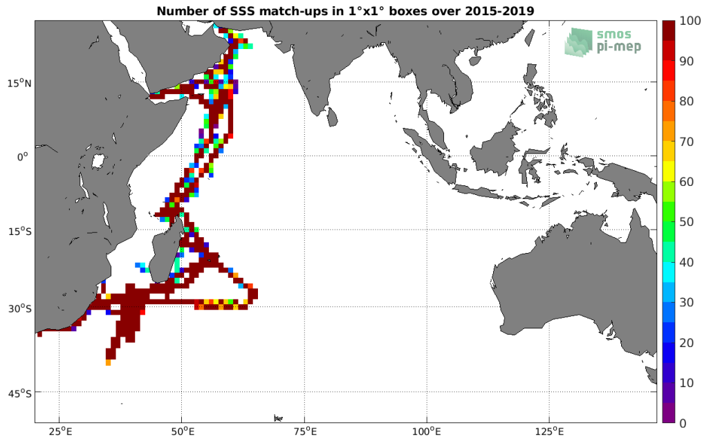
Figure 4: Number of SSS match-ups between TSG (GOSUD-Research-vessel) SSS and the SMAP SSS L3 v4 - 8-Day running (RSS) SSS product for the Indian Ocean Pi-MEP region over 1^\circ \times 1^\circ boxes and for the full satellite product period.
