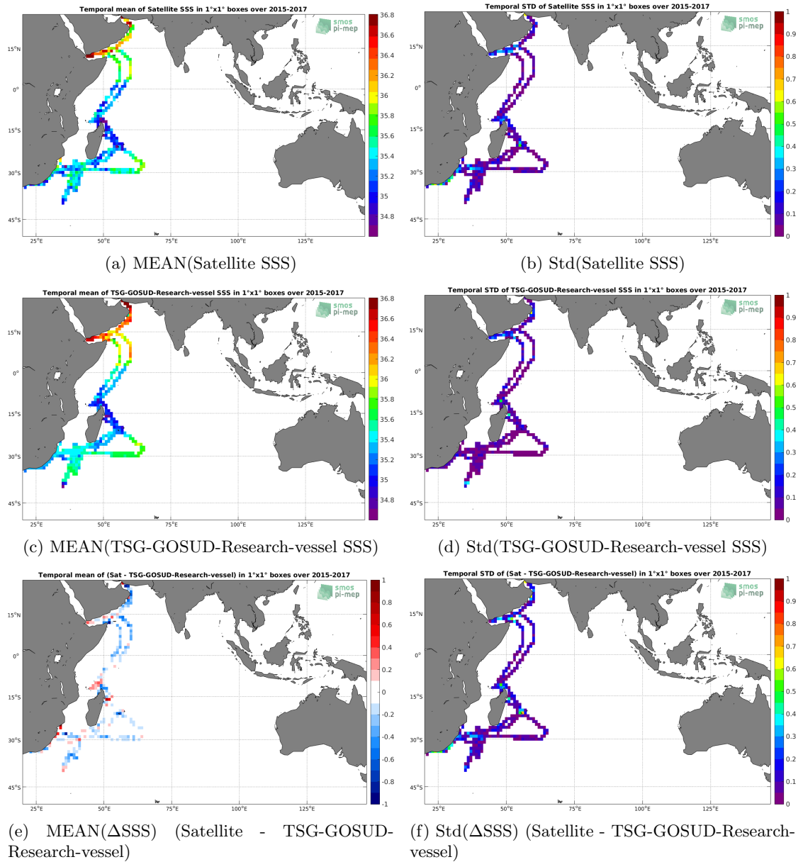
Figure 6: Temporal mean (left) and Std (right) of SSS from SMAP-L3-RSS-V4-8DAY-RUNNING (top), TSG-GOSUD-Research-vessel (middle), and of \Delta SSS (Satellite - TSG-GOSUD-Research-vessel). Only match-up pairs are used to generate these maps.
