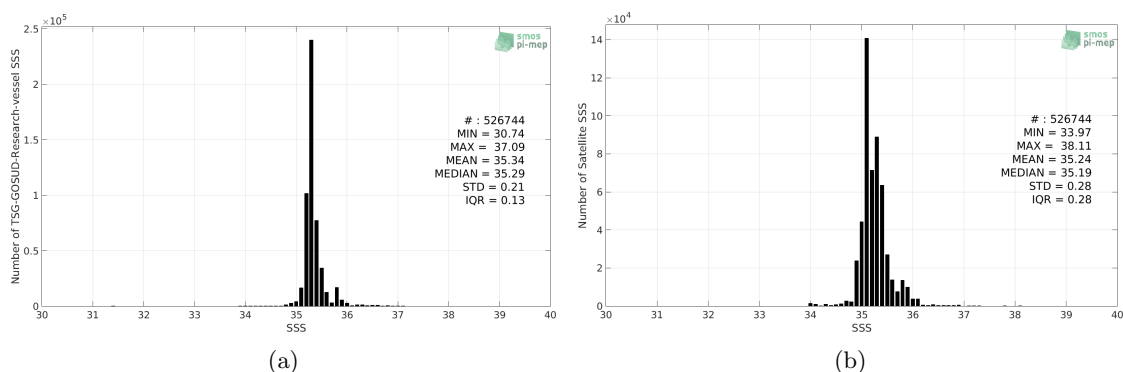
Figure 2: Histograms of SSS from TSG-GOSUD-Research-vessel (a) and SMAP-L3-RSS-V4-8DAY-RUNNING (b) considering all match-up pairs per bins of 0.1 over the Indian Ocean Pi-MEP region and for the full satellite product period.
