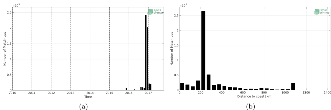
Figure 1: Number of match-ups between TSG-GOSUD-Research-vessel and SMAP-L3-RSS-V4-8DAY-RUNNING SSS as a function of time (a) and as function of the distance to coast (b) over the Indian Ocean Pi-MEP region and for the full satellite product period.
