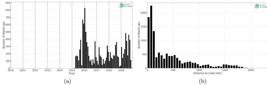
Figure 1: Number of match-ups between Marine mammals and SMAP SSS L3 v4 - 8-Day running (RSS) SSS as a function of time (a) and as function of the distance to coast (b) over the Indian Ocean Pi-MEP region and for the full satellite product period.
