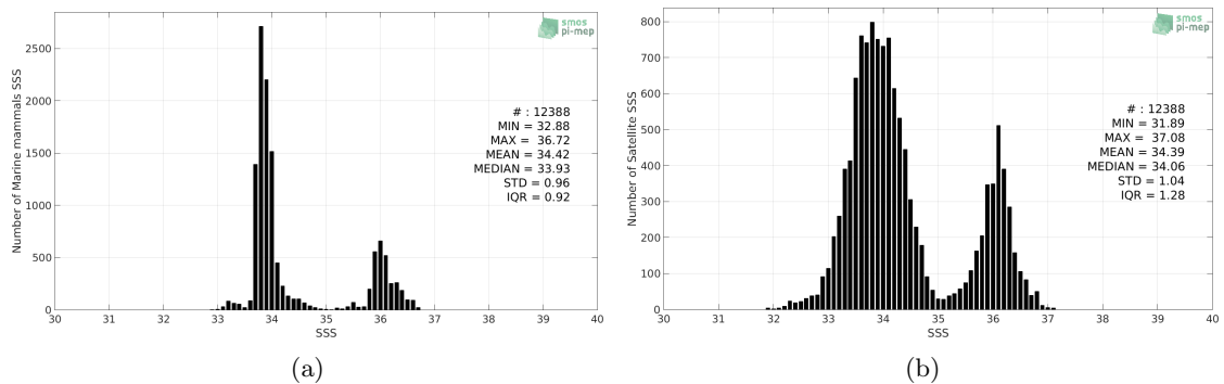
Figure 2: Histograms of SSS from Marine mammals (a) and SMAP SSS L3 v4 - 8-Day running (RSS) (b) considering all match-up pairs per bins of 0.1 over the Indian Ocean Pi-MEP region and for the full satellite product period.
