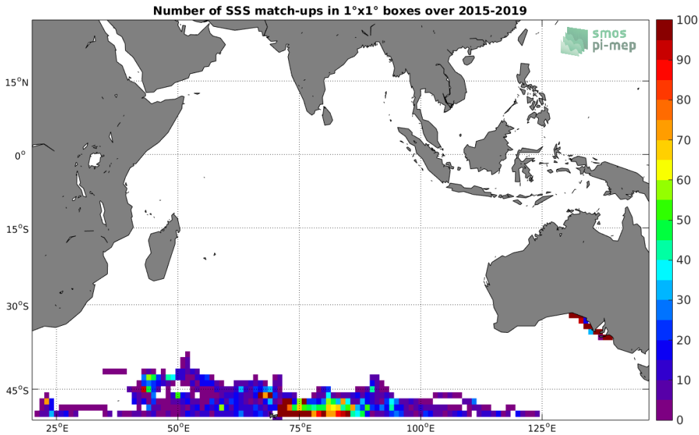
Figure 4: Number of SSS match-ups between Marine mammals SSS and the SMAP SSS L3 v4 - 8-Day running (RSS) SSS product for the Indian Ocean Pi-MEP region over 1^\circ \times 1^\circ boxes and for the full satellite product period.
