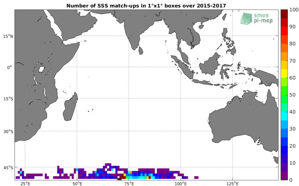
Figure 4: Number of SSS match-ups between Sea mammals SSS and the SMAP-L3-RSS-V4-8DAY-RUNNING SSS product for the Indian Ocean Pi-MEP region over 1^\circ \times 1^\circ boxes and for the full satellite product period.
