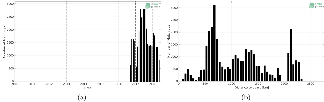
Figure 1: Number of match-ups between Surface drifters and SMAP SSS L3 v4 - 8-Day running (RSS) SSS as a function of time (a) and as function of the distance to coast (b) over the Indian Ocean Pi-MEP region and for the full satellite product period.
