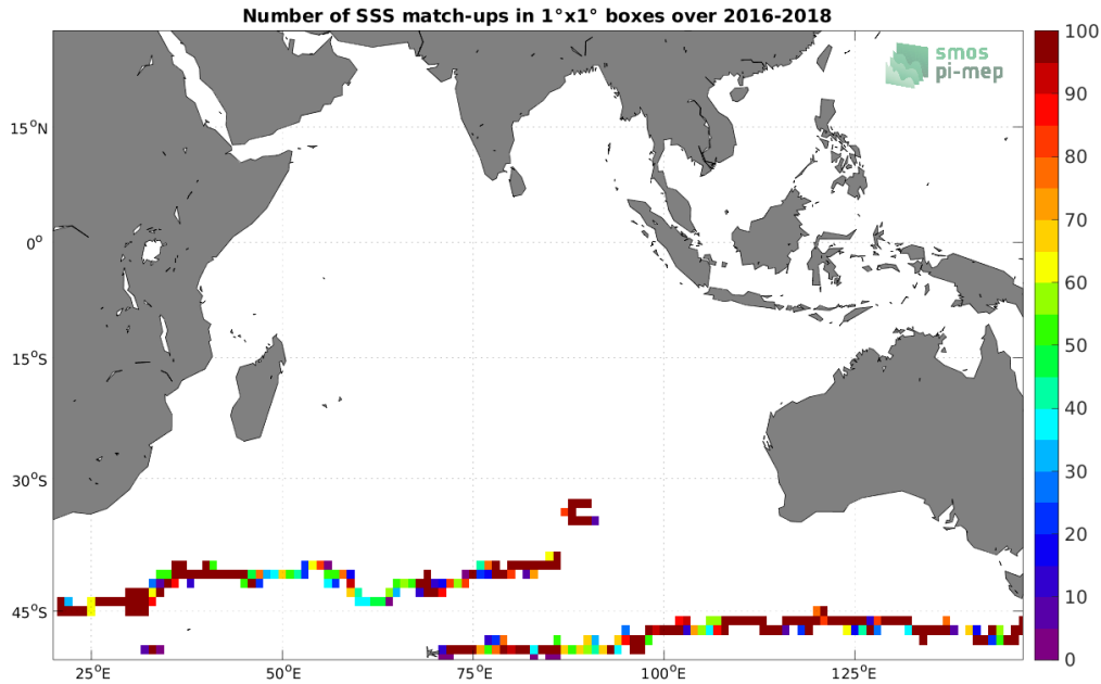
Figure 3: Number of SSS match-ups between Surface drifters SSS and the SMAP SSS L3 v4 - 8-Day running (RSS) SSS product for the Indian Ocean Pi-MEP region over 1^\circ \times 1^\circ boxes and for the full satellite product period.
