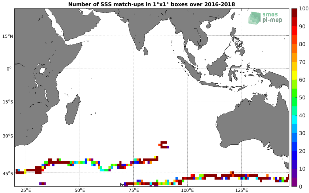
Figure 3: Number of SSS match-ups between Surface drifters SSS and the SMAP SSS L3 v4 - 8-Day running (RSS) SSS product for the Indian Ocean Pi-MEP region over 1°x1° boxes and for the full satellite product period.
