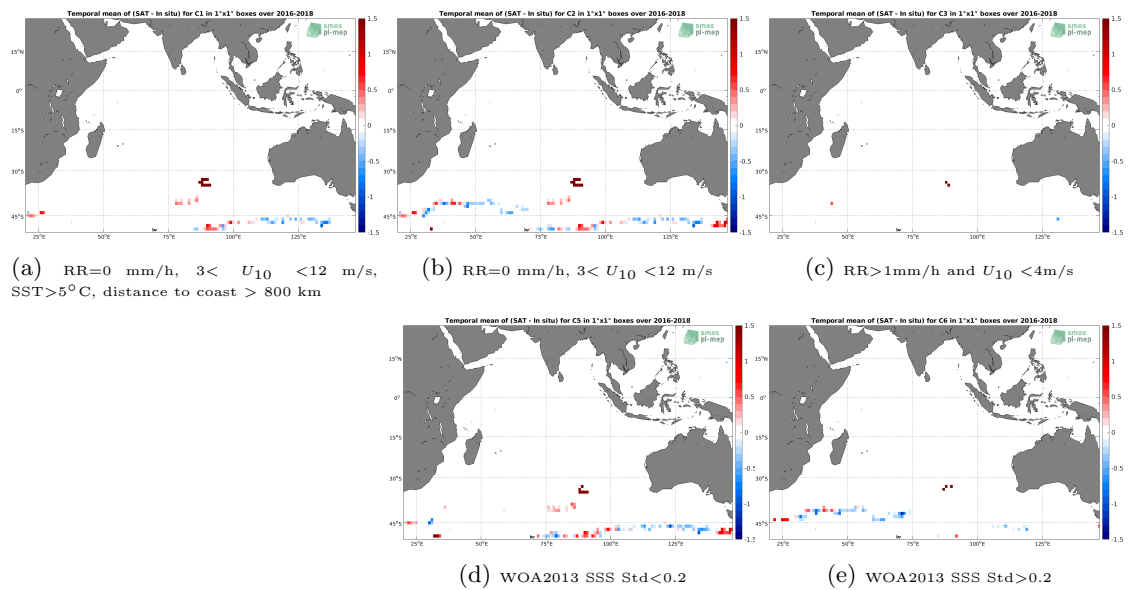
Figure 11: Temporal mean gridded over spatial boxes of size 1°x1° of \Delta SSS (SMAP SSS L3 v4 - 8-Day running (RSS) - Surface drifters) for 5 different subdatasets corresponding to:RR=0 mm/h, 3 < U_{10} < 12 m/s, SST>5°C, distance to coast > 800 km (a), RR=0 mm/h, 3 < U_{10} < 12 m/s (b), RR>1mm/h and U_{10} < 4 m/s (c), WOA2013 SSS Std<0.2 (d), WOA2013 SSS Std>0.2 (e).
