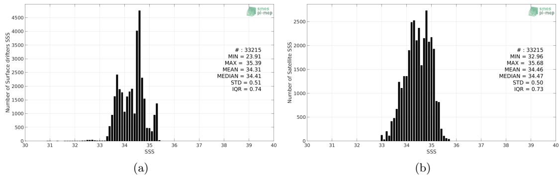
Figure 2: Histograms of SSS from Surface drifters (a) and SMAP-L3-RSS-V4-8DAY-RUNNING (b) considering all match-up pairs per bins of 0.1 over the Indian Ocean Pi-MEP region and for the full satellite product period.
