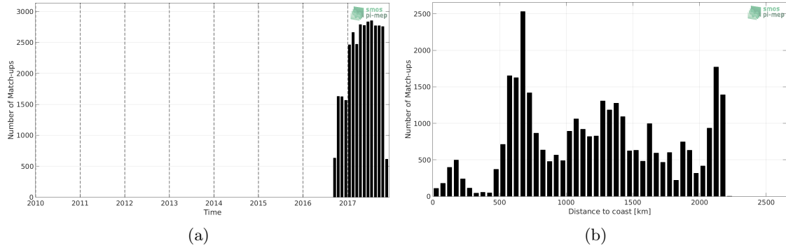
Figure 1: Number of match-ups between Surface drifters and SMAP-L3-RSS-V4-8DAY-RUNNING SSS as a function of time (a) and as function of the distance to coast (b) over the Indian Ocean Pi-MEP region and for the full satellite product period.
