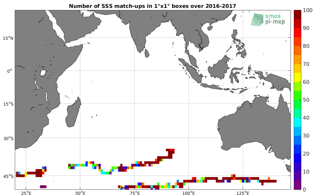
Figure 3: Number of SSS match-ups between Surface drifters SSS and the SMAP-L3-RSS-V4-8DAY-RUNNING SSS product for the Indian Ocean Pi-MEP region over 1°x1° boxes and for the full satellite product period.
