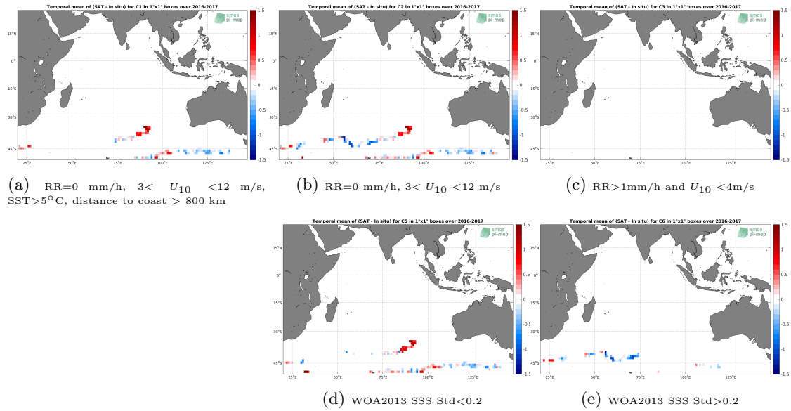
Figure 11: Temporal mean gridded over spatial boxes of size 1^\circ \times 1^\circ of \Delta SSS (SMAP-L3-RSS-V4-8DAY-RUNNING - Surface drifters) for 5 different subdatasets corresponding to:RR=0 mm/h, 3 < U_{10} < 12 m/s, SST >5^\circ C, distance to coast > 800 km (a), RR=0 mm/h, 3 < U_{10} < 12 m/s (b), RR >1 mm/h and U_{10} < 4 m/s (c), WOA2013 SSS Std <0.2 (d), WOA2013 SSS Std >0.2 (e).
