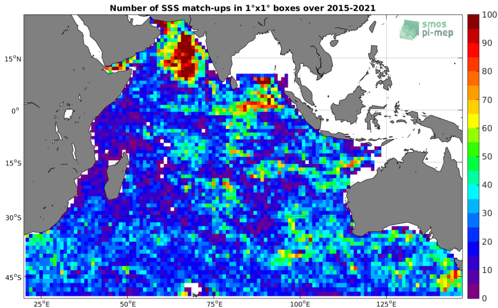
Figure 4: Number of SSS match-ups between Argo SSS and the SMAP SSS L3 v4 - 8-Day running (RSS) SSS product for the Indian Ocean Pi-MEP region over 1^\circ \times 1^\circ boxes and for the full satellite product period.
