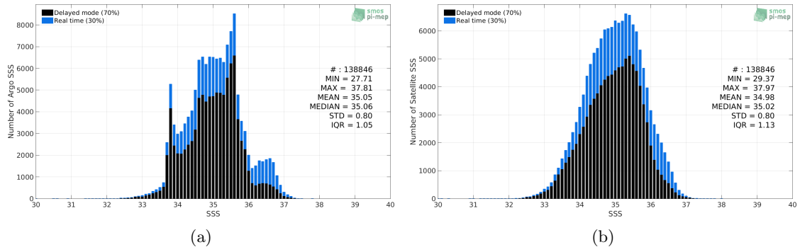
Figure 2: Histograms of SSS from Argo (a) and SMAP SSS L3 v4 - 8-Day running (RSS) (b) considering all match-up pairs per bins of 0.1 over the Indian Ocean Pi-MEP region and for the full satellite product period.
