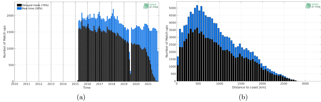
Figure 1: Number of match-ups between Argo and SMAP SSS L3 v4 - 8-Day running (RSS) SSS as a function of time (a) and as function of the distance to coast (b) over the Indian Ocean Pi-MEP region and for the full satellite product period.
