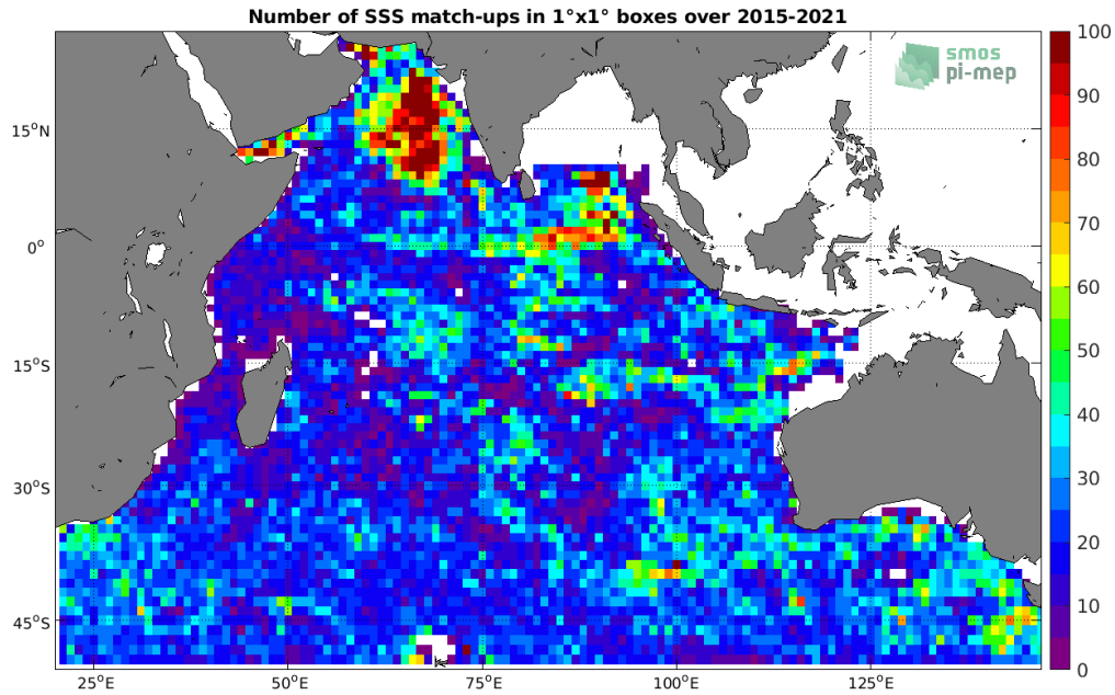
Figure 4: Number of SSS match-ups between Argo SSS and the SMAP SSS L3 v4 - 8-Day running (RSS) SSS product for the Indian Ocean Pi-MEP region over 1^\circ \times 1^\circ boxes and for the full satellite product period.
