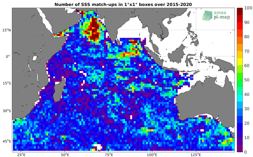
Figure 4: Number of SSS match-ups between Argo SSS and the SMAP SSS L3 v4 - 8-Day running (RSS) SSS product for the Indian Ocean Pi-MEP region over 1°x1° boxes and for the full satellite product period.
