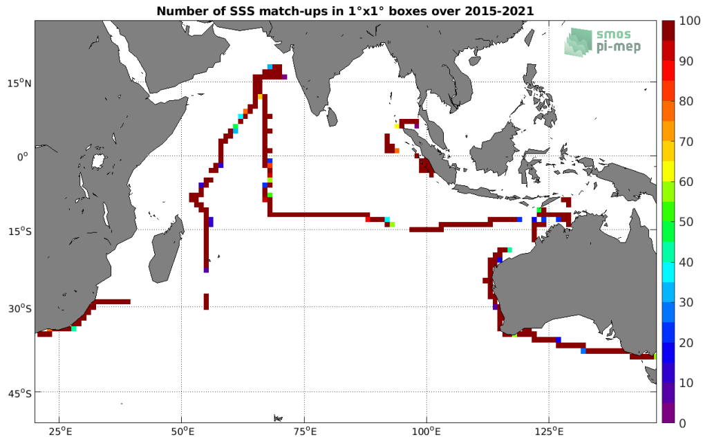
Figure 4: Number of SSS match-ups between TSG (SAMOS) SSS and the SMAP SSS L3 v4 - Monthly (RSS) SSS product for the Indian Ocean Pi-MEP region over 1^\circ \times 1^\circ boxes and for the full satellite product period.
