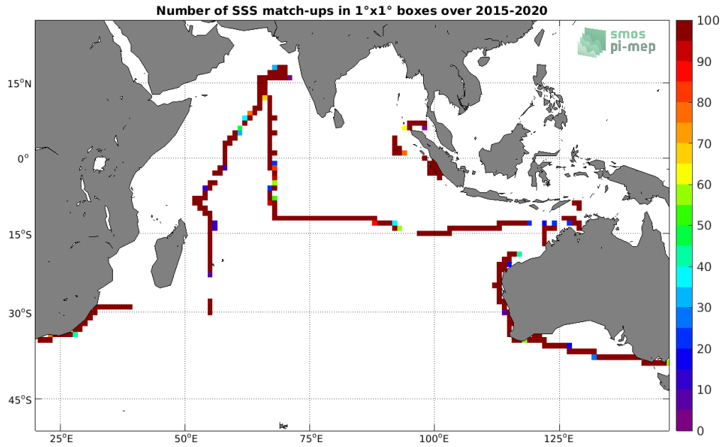
Figure 4: Number of SSS match-ups between TSG (SAMOS) SSS and the SMAP SSS L3 v4 - Monthly (RSS) SSS product for the Indian Ocean Pi-MEP region over 1°x1° boxes and for the full satellite product period.
