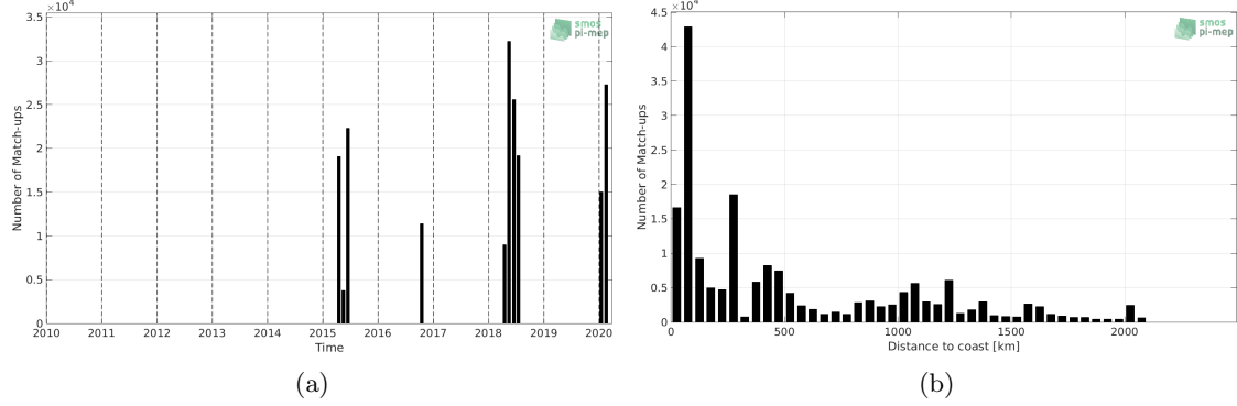
Figure 1: Number of match-ups between TSG-SAMOS and SMAP-L3-RSS-V4-MONTHLY SSS as a function of time (a) and as function of the distance to coast (b) over the Indian Ocean Pi-MEP region and for the full satellite product period.
