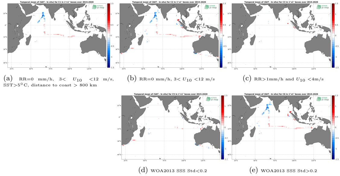
Figure 12: Temporal mean gridded over spatial boxes of size 1^\circ \times 1^\circ of \Delta SSS (SMAP-L3-RSS-V4-MONTHLY - TSG-SAMOS) for 5 different subdatasets corresponding to: RR=0 mm/h, 3 < U_{10} < 12 m/s, SST >5^\circ C, distance to coast > 800 km (a), RR=0 mm/h, 3 < U_{10} < 12 m/s (b), RR >1 mm/h and U_{10} < 4 m/s (c), WOA2013 SSS Std <0.2 (d), WOA2013 SSS Std >0.2 (e).
