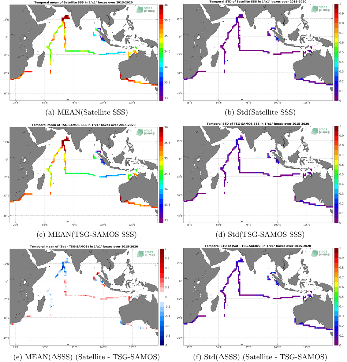
Figure 6: Temporal mean (left) and Std (right) of SSS from SMAP-L3-RSS-V4-MONTHLY (top), TSG-SAMOS (middle), and of \Delta SSS (Satellite - TSG-SAMOS). Only match-up pairs are used to generate these maps.
