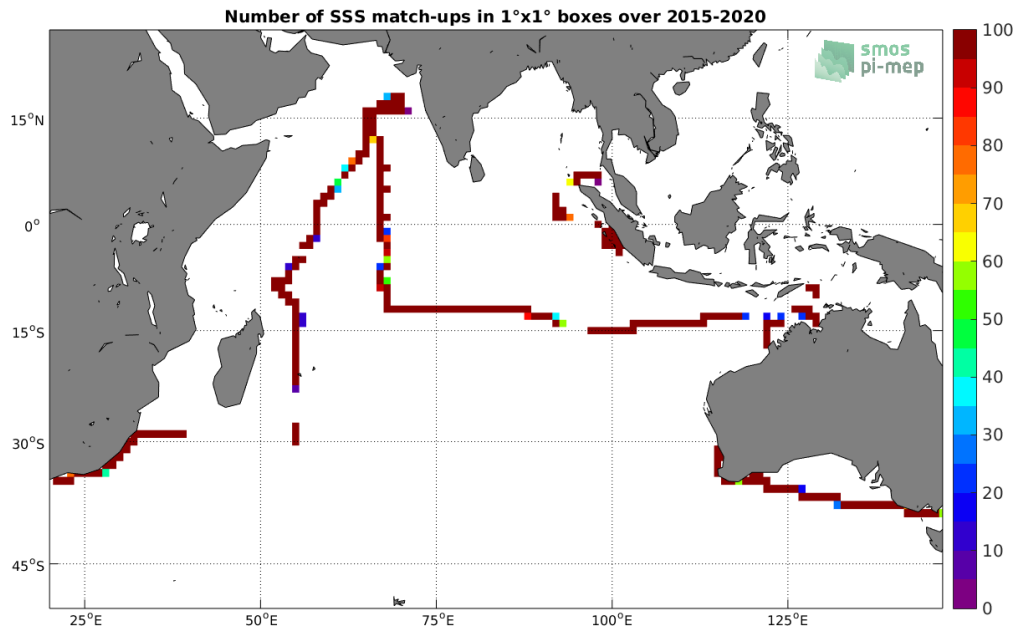
Figure 4: Number of SSS match-ups between TSG-SAMOS SSS and the SMAP-L3-RSS-V4-MONTHLY SSS product for the Indian Ocean Pi-MEP region over 1^\circ \times 1^\circ boxes and for the full satellite product period.
