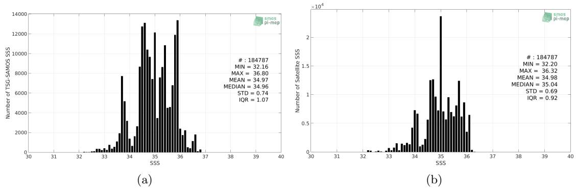
Figure 2: Histograms of SSS from TSG-SAMOS (a) and SMAP-L3-RSS-V4-MONTHLY (b) considering all match-up pairs per bins of 0.1 over the Indian Ocean Pi-MEP region and for the full satellite product period.
