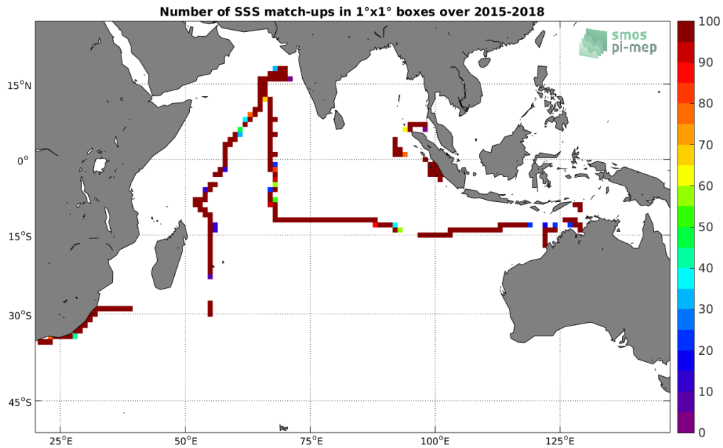
Figure 4: Number of SSS match-ups between TSG-SAMOS SSS and the SMAP-L3-RSS-V4-MONTHLY SSS product for the Indian Ocean Pi-MEP region over 1°x1° boxes and for the full satellite product period.
