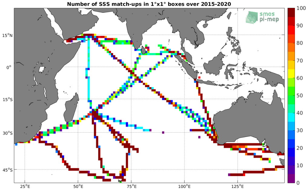
Figure 4: Number of SSS match-ups between TSG (LEGOS-DM) SSS and the SMAP SSS L3 v4 - Monthly (RSS) SSS product for the Indian Ocean Pi-MEP region over 1^\circ \times 1^\circ boxes and for the full satellite product period.
