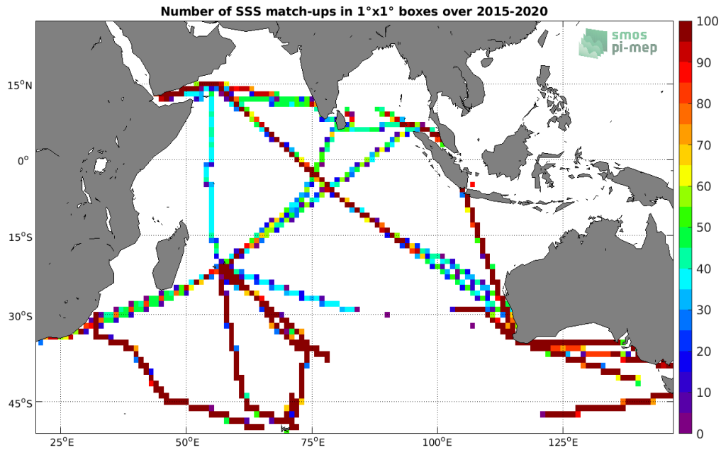
Figure 4: Number of SSS match-ups between TSG (LEGOS-DM) SSS and the SMAP SSS L3 v4 - Monthly (RSS) SSS product for the Indian Ocean Pi-MEP region over 1^\circ \times 1^\circ boxes and for the full satellite product period.
