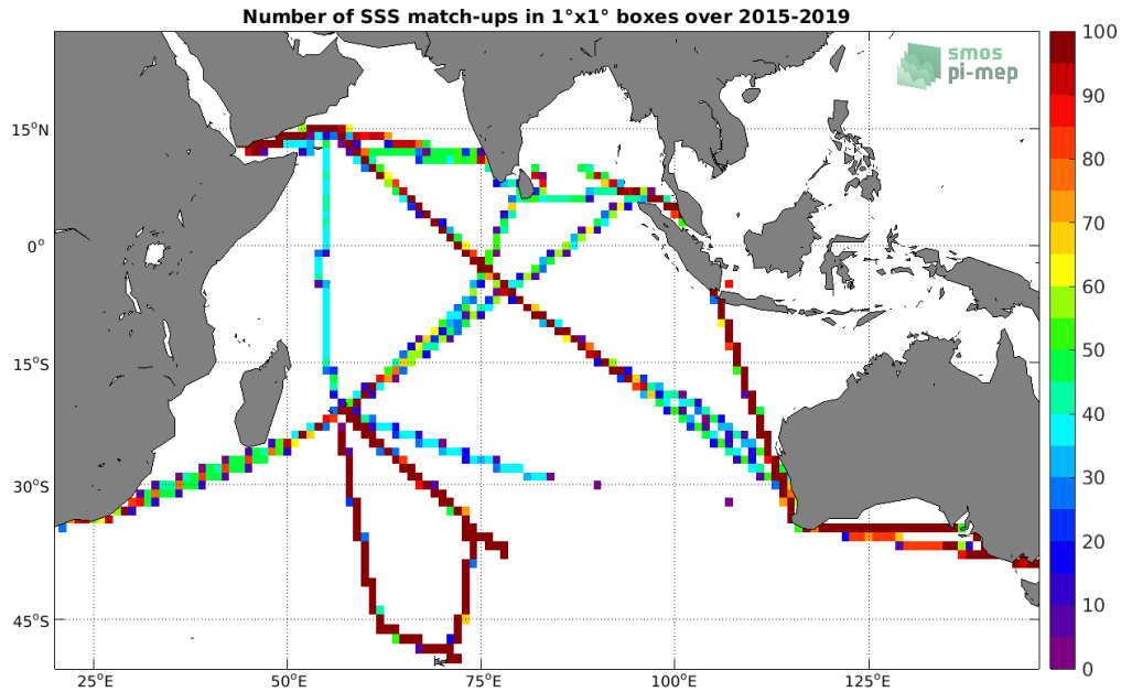
Figure 4: Number of SSS match-ups between TSG (LEGOS-DM) SSS and the SMAP SSS L3 v4 - Monthly (RSS) SSS product for the Indian Ocean Pi-MEP region over 1°x1° boxes and for the full satellite product period.
