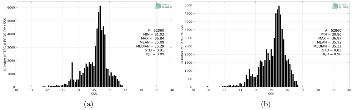
Figure 2: Histograms of SSS from TSG (LEGOS-DM) (a) and SMAP SSS L3 v4 - Monthly (RSS) (b) considering all match-up pairs per bins of 0.1 over the Indian Ocean Pi-MEP region and for the full satellite product period.
