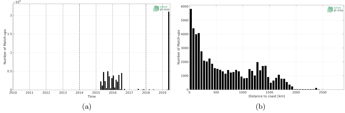
Figure 1: Number of match-ups between TSG (LEGOS-DM) and SMAP SSS L3 v4 - Monthly (RSS) SSS as a function of time (a) and as function of the distance to coast (b) over the Indian Ocean Pi-MEP region and for the full satellite product period.
