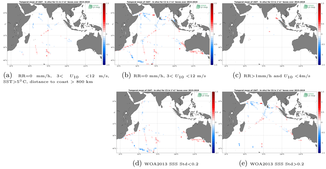
Figure 12: Temporal mean gridded over spatial boxes of size 1^\circ \times 1^\circ of \Delta SSS (SMAP-L3-RSS-V4-MONTHLY - TSG-LEGOS-DM) for 5 different subdatasets corresponding to: RR=0 mm/h, 3 < U_{10} < 12 m/s, SST > 5^\circ C , distance to coast > 800 km (a), RR=0 mm/h, 3 < U_{10} < 12 m/s (b), RR > 1 mm/h and U_{10} < 4 m/s (c), WOA2013 SSS Std < 0.2 (d), WOA2013 SSS Std > 0.2 (e).
