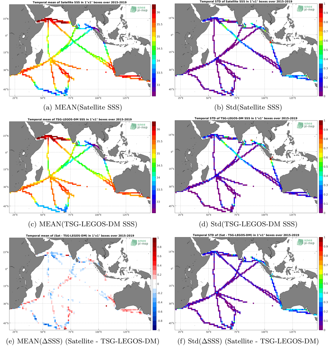
Figure 6: Temporal mean (left) and Std (right) of SSS from SMAP-L3-RSS-V4-MONTHLY (top), TSG-LEGOS-DM (middle), and of \Delta SSS (Satellite - TSG-LEGOS-DM). Only match-up pairs are used to generate these maps.
