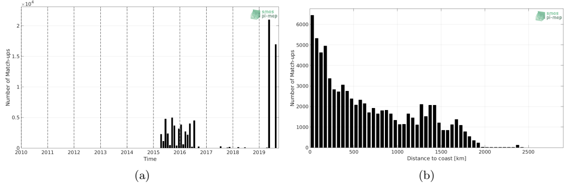
Figure 1: Number of match-ups between TSG-LEGOS-DM and SMAP-L3-RSS-V4-MONTHLY SSS as a function of time (a) and as function of the distance to coast (b) over the Indian Ocean Pi-MEP region and for the full satellite product period.
