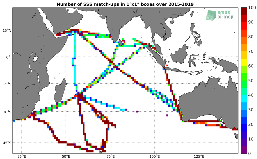
Figure 4: Number of SSS match-ups between TSG-LEGOS-DM SSS and the SMAP-L3-RSS-V4-MONTHLY SSS product for the Indian Ocean Pi-MEP region over 1^\circ \times 1^\circ boxes and for the full satellite product period.
