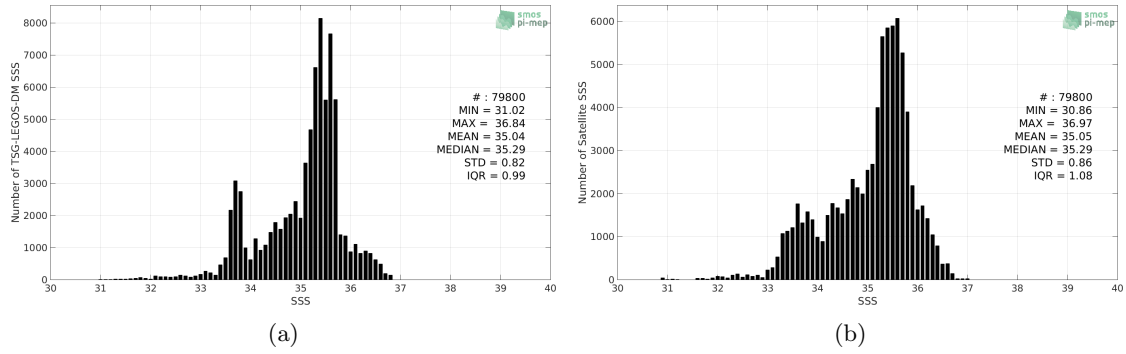
Figure 2: Histograms of SSS from TSG-LEGOS-DM (a) and SMAP-L3-RSS-V4-MONTHLY (b) considering all match-up pairs per bins of 0.1 over the Indian Ocean Pi-MEP region and for the full satellite product period.
