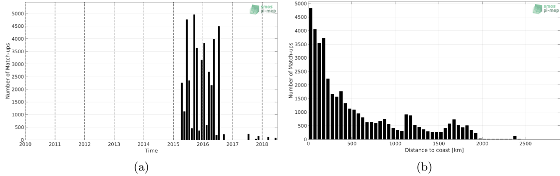
Figure 1: Number of match-ups between TSG-LEGOS-DM and SMAP-L3-RSS-V4-MONTHLY SSS as a function of time (a) and as function of the distance to coast (b) over the Indian Ocean Pi-MEP region and for the full satellite product period.
