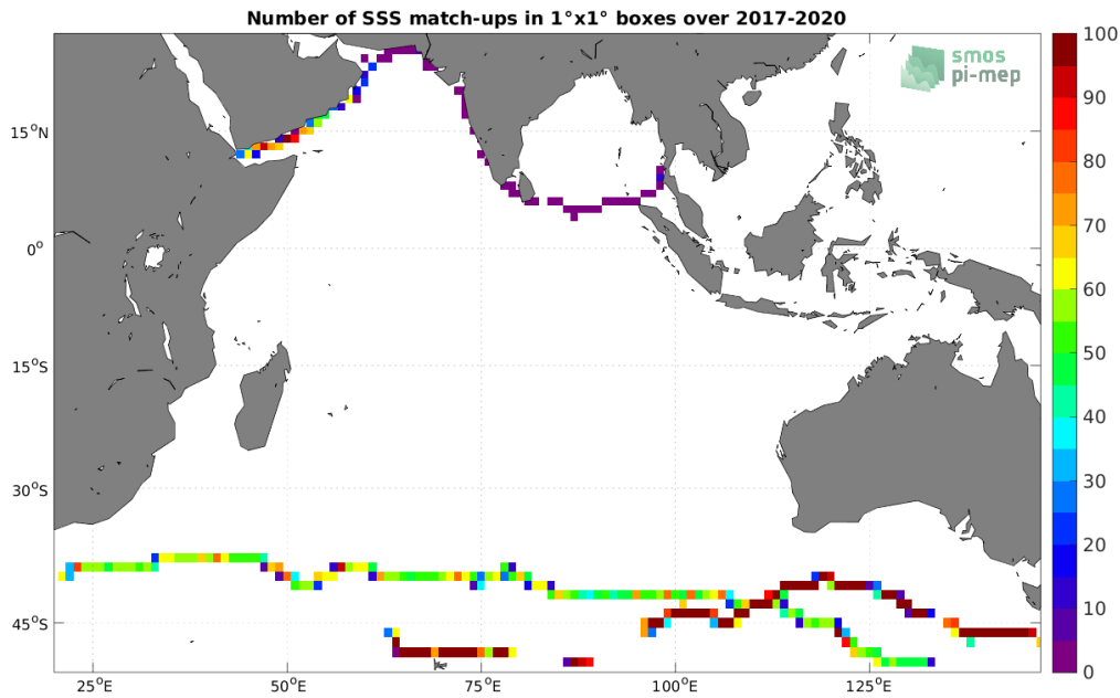
Figure 4: Number of SSS match-ups between TSG (GOSUD-Sailing-ship) SSS and the SMAP SSS L3 v4 - Monthly (RSS) SSS product for the Indian Ocean Pi-MEP region over 1^\circ \times 1^\circ boxes and for the full satellite product period.
