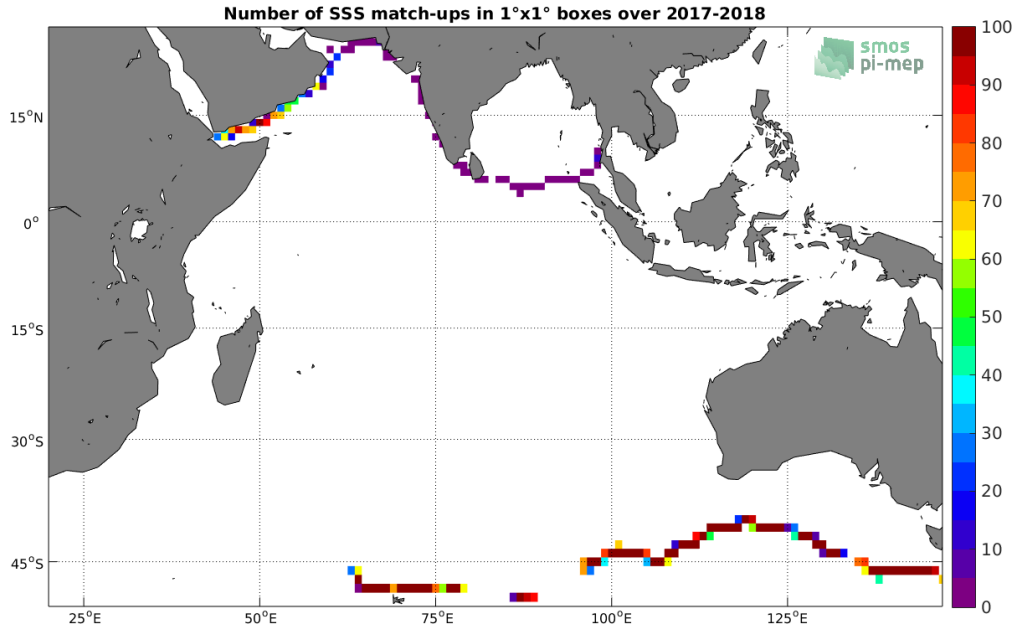
Figure 4: Number of SSS match-ups between TSG (GOSUD-Sailing-ship) SSS and the SMAP SSS L3 v4 - Monthly (RSS) SSS product for the Indian Ocean Pi-MEP region over 1^\circ \times 1^\circ boxes and for the full satellite product period.
