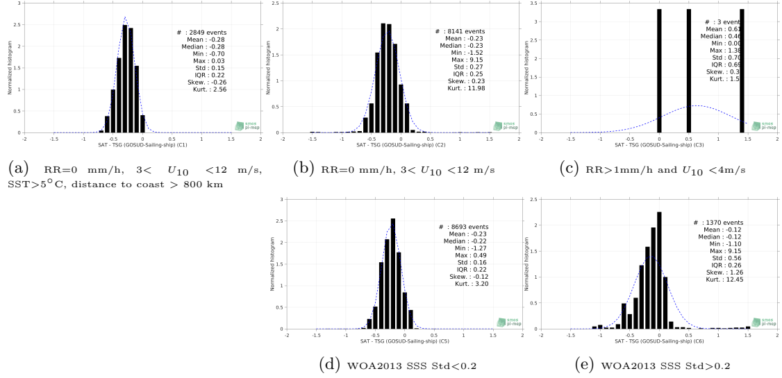
Figure 13: Normalized histogram of \Delta SSS (SMAP SSS L3 v4 - Monthly (RSS) - TSG (GOSUD-Sailing-ship)) for 5 different subdatasets corresponding to: RR=0 mm/h, 3 < U_{10} < 12 m/s, SST>5°C, distance to coast > 800 km (a), RR=0 mm/h, 3 < U_{10} < 12 m/s (b), RR>1mm/h and U_{10} < 4 m/s (c), WOA2013 SSS Std<0.2 (d), WOA2013 SSS Std>0.2 (e).
