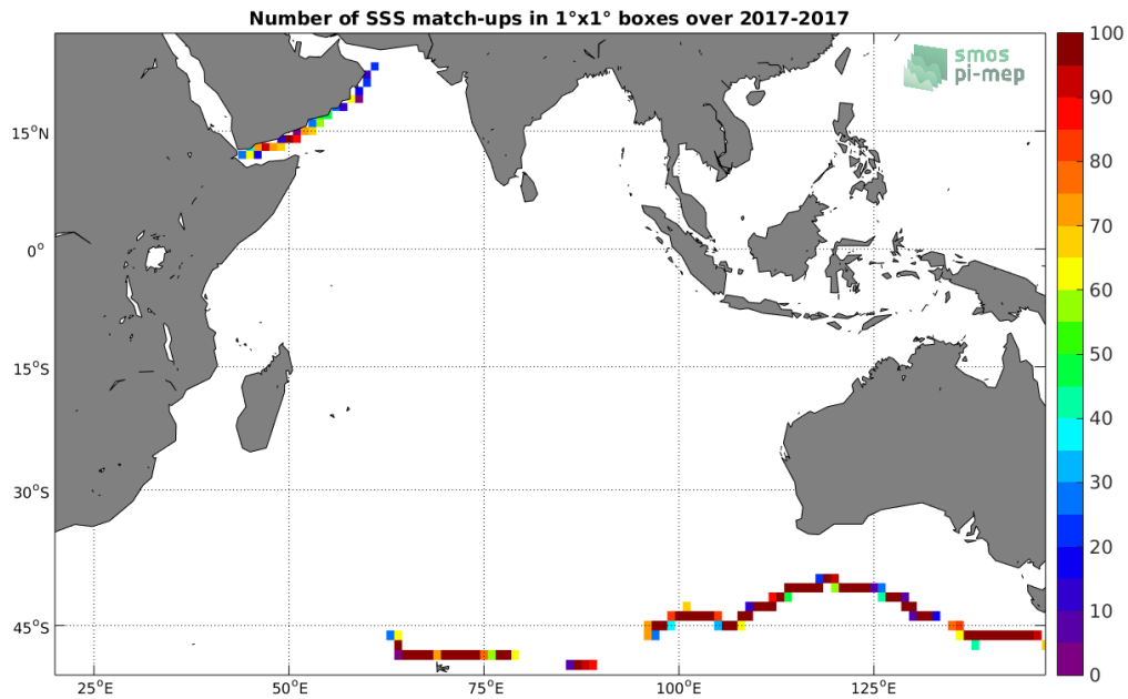
Figure 4: Number of SSS match-ups between TSG-GOSUD-Sailing-ship SSS and the SMAP-L3-RSS-V4-MONTHLY SSS product for the Indian Ocean Pi-MEP region over 1°x1° boxes and for the full satellite product period.
