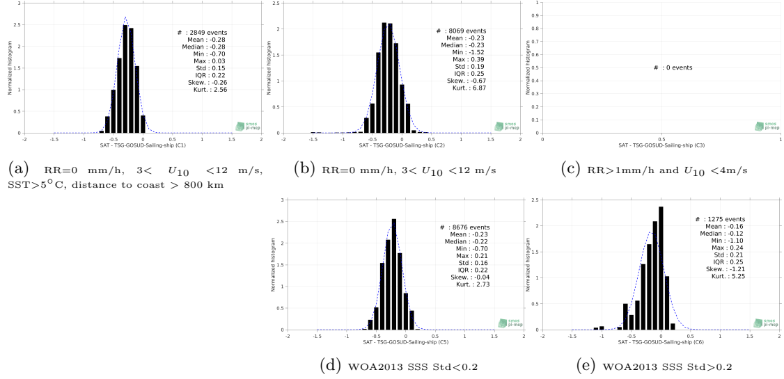
Figure 13: Normalized histogram of \Delta\text{SSS} (SMAP-L3-RSS-V4-MONTHLY - TSG-GOSUD-Sailing-ship) for 5 different subdatasets corresponding to: RR=0 mm/h, 3 < U_{10} < 12 m/s, SST > 5^{\circ}\text{C} , distance to coast > 800 km (a), RR=0 mm/h, 3 < U_{10} < 12 m/s (b), RR > 1\text{mm/h} and U_{10} < 4\text{m/s} (c), WOA2013 SSS Std < 0.2 (d), WOA2013 SSS Std > 0.2 (e).
