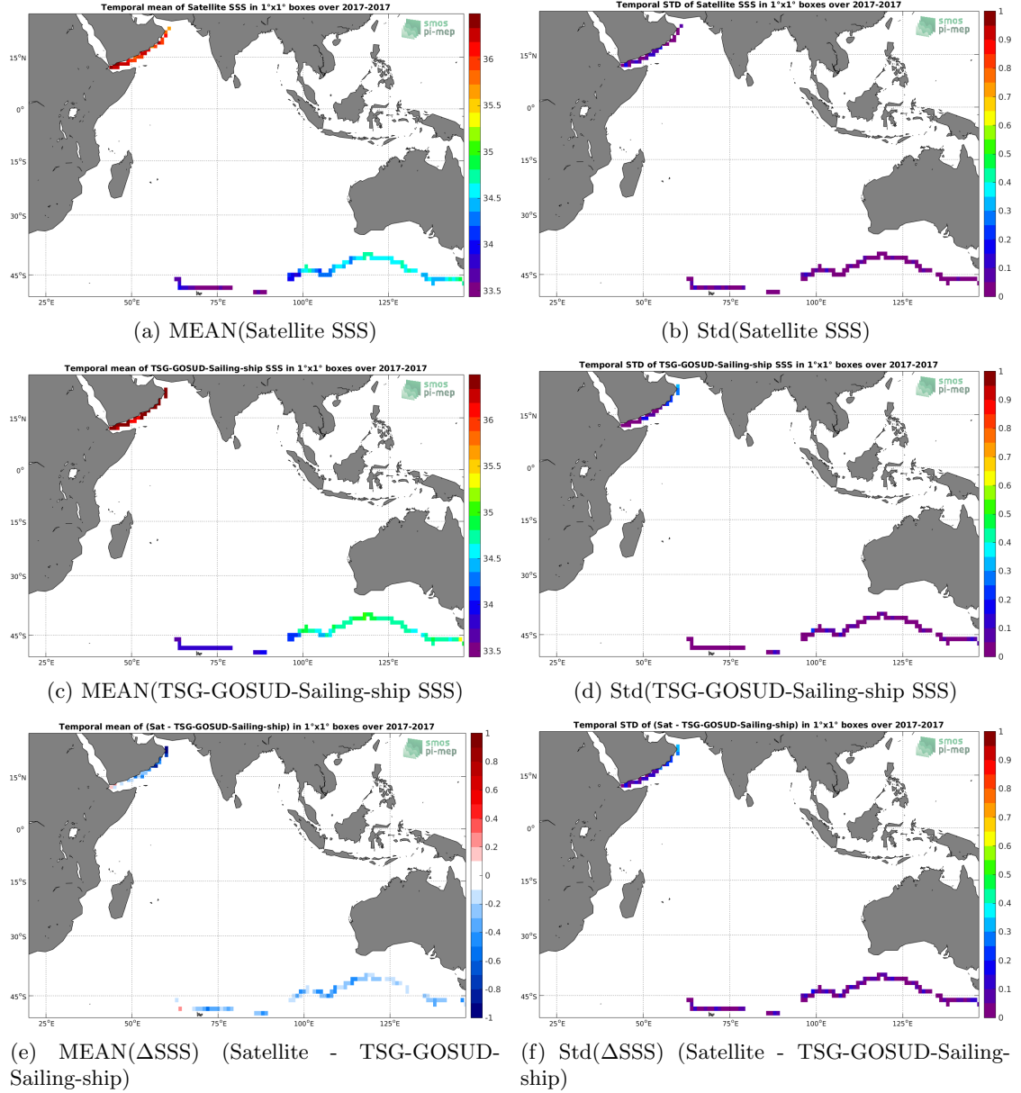
Figure 6: Temporal mean (left) and Std (right) of SSS from SMAP-L3-RSS-V4-MONTHLY (top), TSG-GOSUD-Sailing-ship (middle), and of \Delta SSS (Satellite - TSG-GOSUD-Sailing-ship). Only match-up pairs are used to generate these maps.
