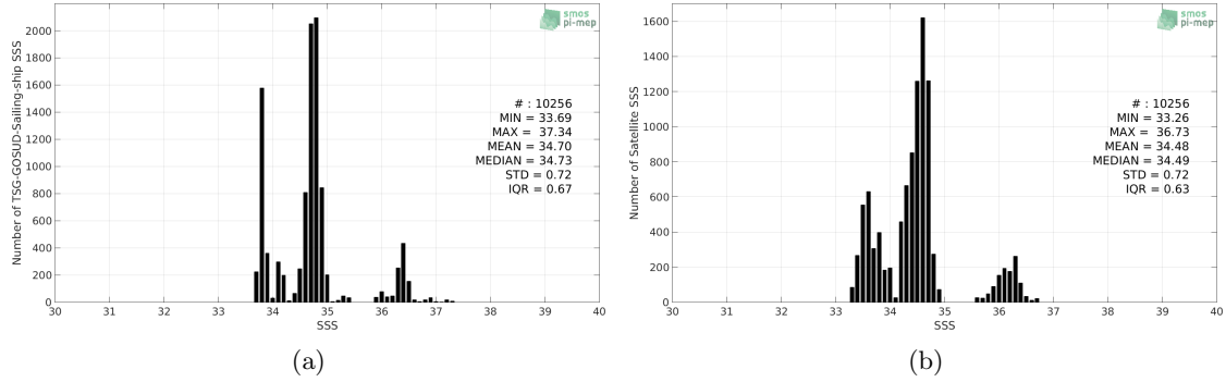
Figure 2: Histograms of SSS from TSG-GOSUD-Sailing-ship (a) and SMAP-L3-RSS-V4-MONTHLY (b) considering all match-up pairs per bins of 0.1 over the Indian Ocean Pi-MEP region and for the full satellite product period.
