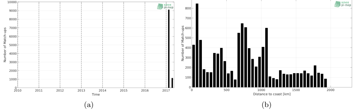
Figure 1: Number of match-ups between TSG-GOSUD-Sailing-ship and SMAP-L3-RSS-V4-MONTHLY SSS as a function of time (a) and as function of the distance to coast (b) over the Indian Ocean Pi-MEP region and for the full satellite product period.
