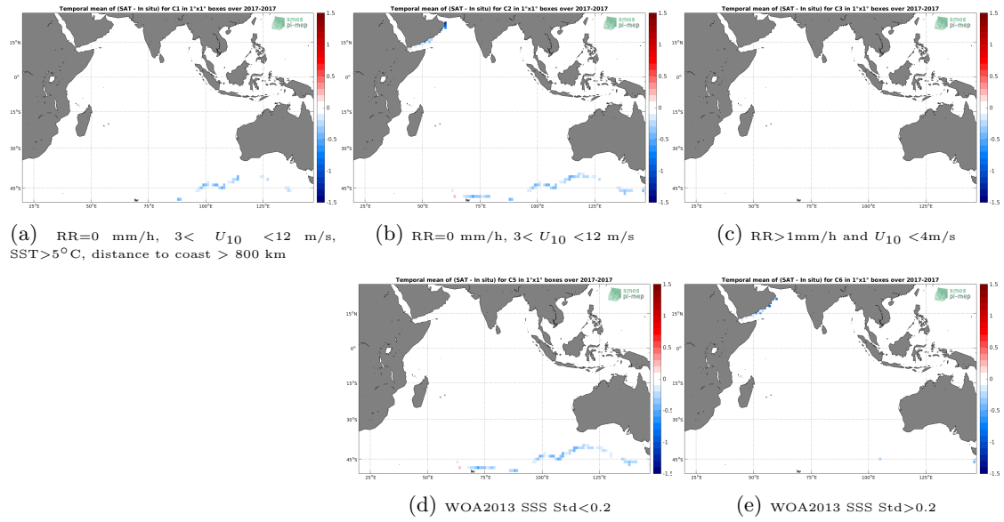
Figure 12: Temporal mean gridded over spatial boxes of size 1^\circ \times 1^\circ of \Delta SSS (SMAP-L3-RSS-V4-MONTHLY - TSG-GOSUD-Sailing-ship) for 5 different subdatasets corresponding to: RR=0 mm/h, 3 < U_{10} < 12 m/s, SST >5^\circ C, distance to coast > 800 km (a), RR=0 mm/h, 3 < U_{10} < 12 m/s (b), RR >1 mm/h and U_{10} < 4 m/s (c), WOA2013 SSS Std <0.2 (d), WOA2013 SSS Std >0.2 (e).
