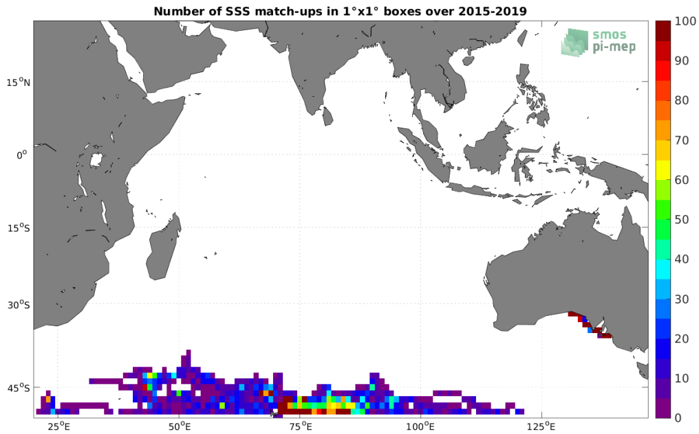
Figure 4: Number of SSS match-ups between Marine mammals SSS and the SMAP SSS L3 v4 - Monthly (RSS) SSS product for the Indian Ocean Pi-MEP region over 1^\circ \times 1^\circ boxes and for the full satellite product period.
